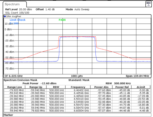
802.11ax (40MHz) 6525MHz Chain D NSS-2
