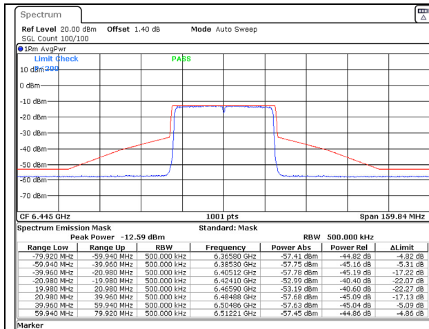
802.11ax (40MHz) 6445MHz Chain C NSS-2
