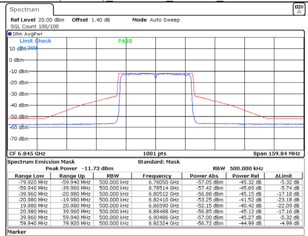
802.11ax (40MHz) 6845MHz Chain D NSS-2
