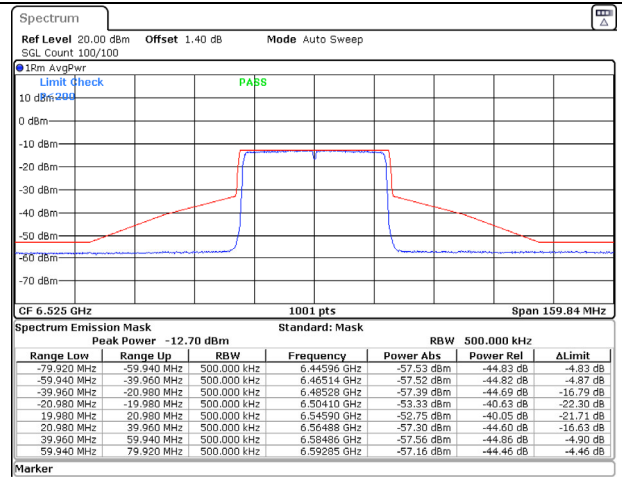
802.11ax (40MHz) 6525MHz Chain B NSS-2
