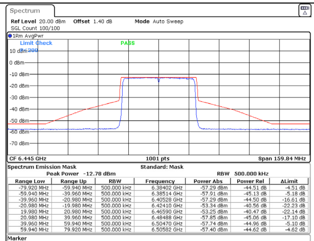
802.11ax (40MHz) 6445MHz Chain D NSS-2
