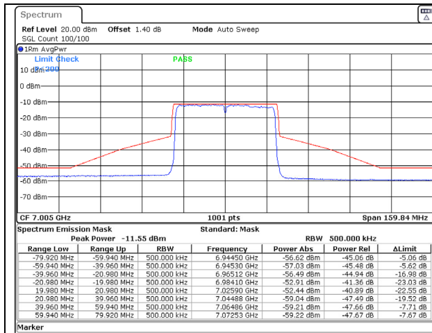
802.11ax (40MHz) 7005MHz Chain A NSS-2
