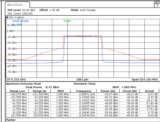
802.11ax (80MHz) 6225MHz Chain B NSS-2
