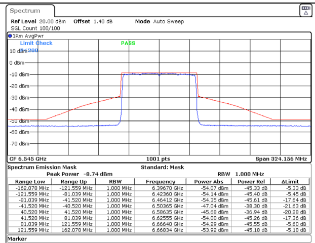
802.11ax (80MHz) 6545MHz Chain B NSS-2
