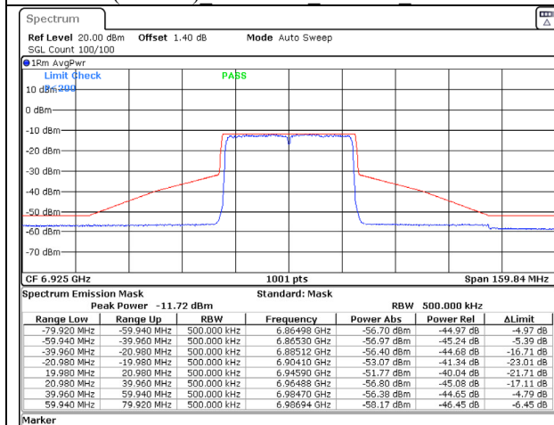
802.11ax (40MHz) 6925MHz Chain A NSS-2
