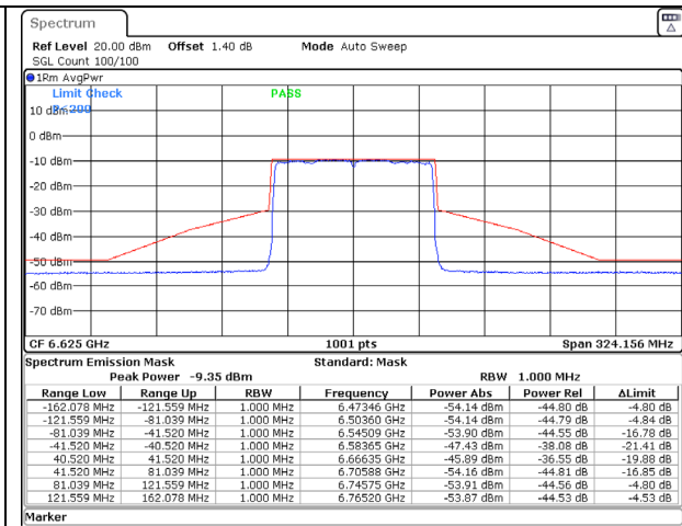
802.11ax (80MHz) 6625MHz Chain D NSS-2
