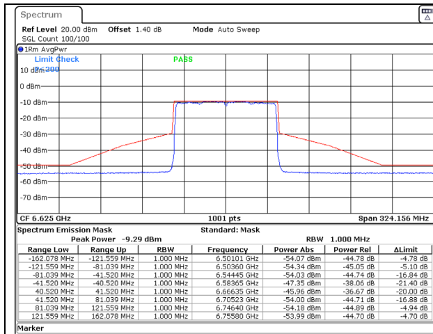
802.11ax (80MHz) 6625MHz Chain C NSS-2
