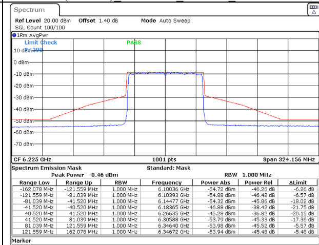
802.11ax (80MHz) 6225MHz Chain D NSS-2
