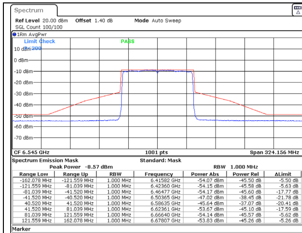
802.11ax (80MHz) 6545MHz Chain A NSS-2
