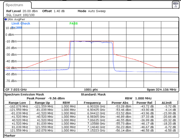
802.11ax (80MHz) 7025MHz Chain D NSS-2
