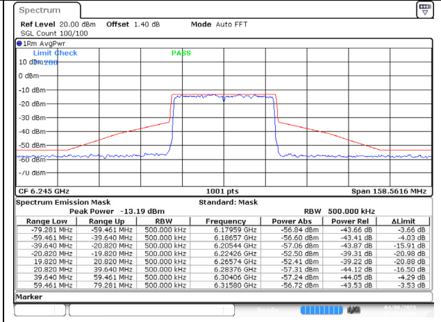
802.11ax (40MHz) 6245MHz Chain D NSS-1
