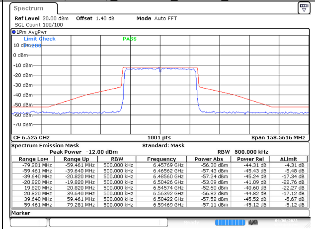
802.11ax (40MHz) 6525MHz Chain B NSS-1
