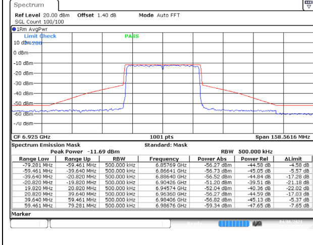
802.11ax (40MHz) 6925MHz Chain C NSS-1
