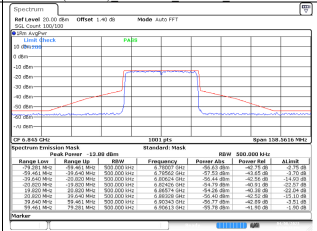
802.11ax (40MHz) 6845MHz Chain B NSS-1
