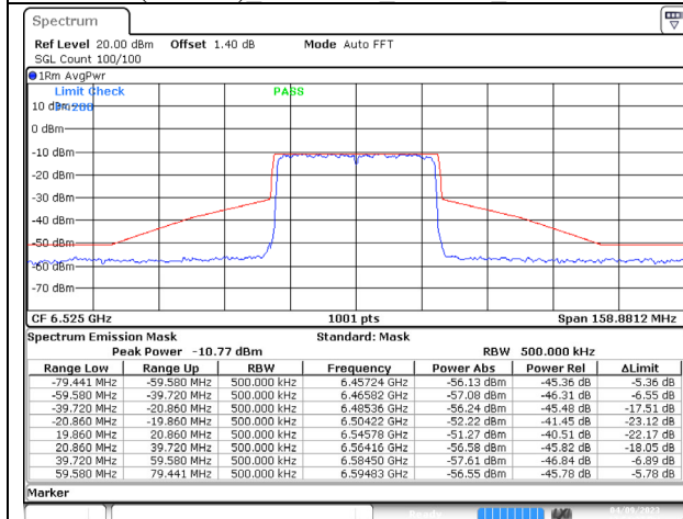
802.11ax (40MHz) 6525MHz Chain C NSS-4
