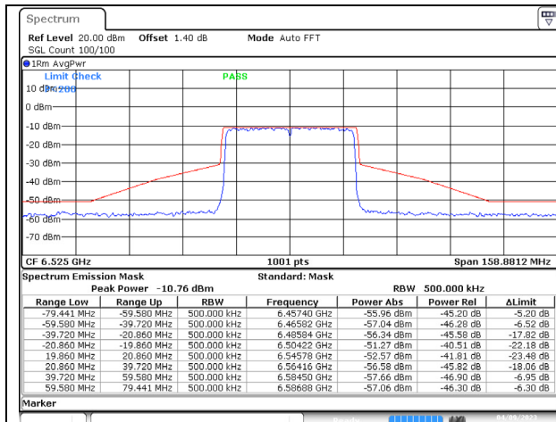
802.11ax (40MHz) 6525MHz Chain A NSS-4
