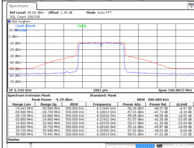
802.11ax (40MHz) 6245MHz Chain A NSS-4
