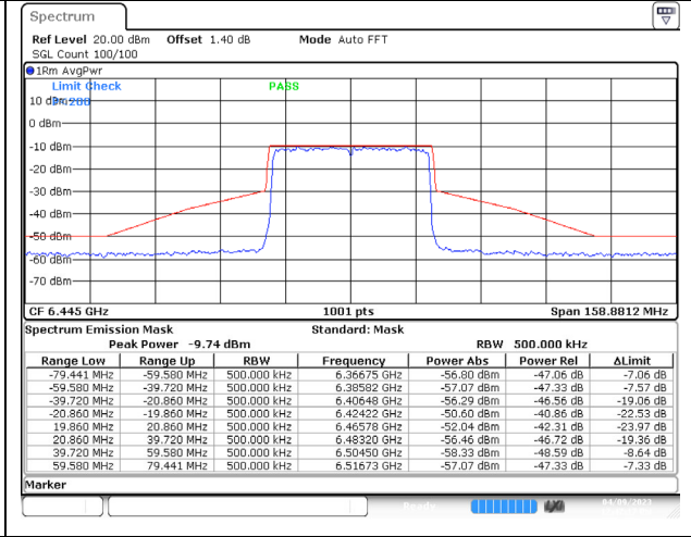
802.11ax (40MHz) 6445MHz Chain B NSS-4
