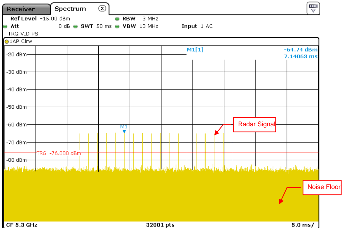
Radar Signal 0
