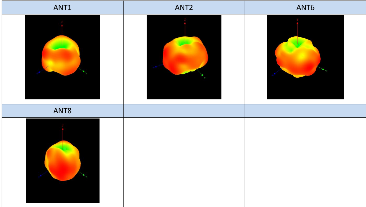
Figure33 2.4G 3D far-field pattern
