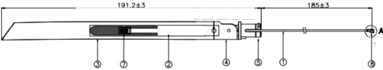
Figure9 ANT8sketch map
