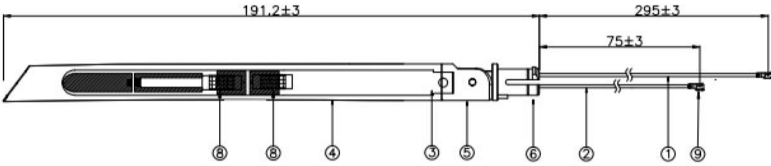
Figure5 ANT2&ANT3sketch map
