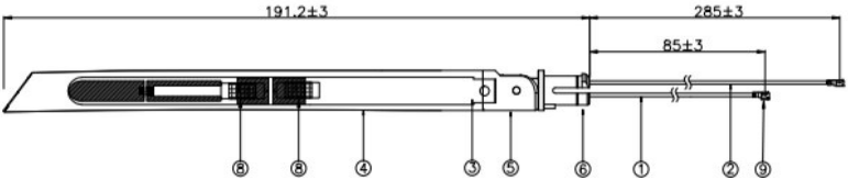
Figure8 ANT6&ANT7sketch map
