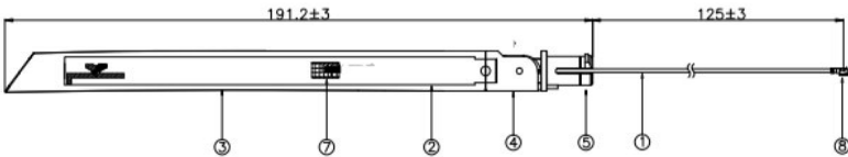
Figure6 ANT4sketch map
