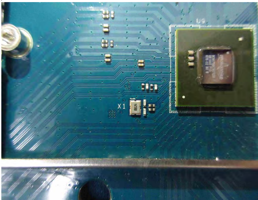
(26) EUT Photo
