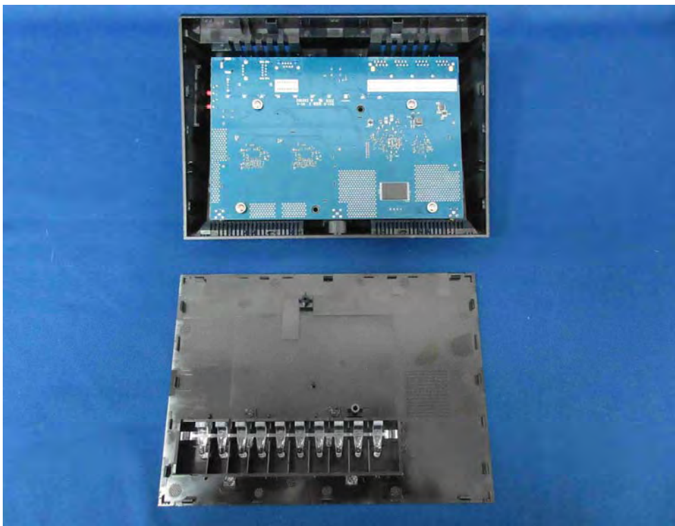
(1) EUT Photo
