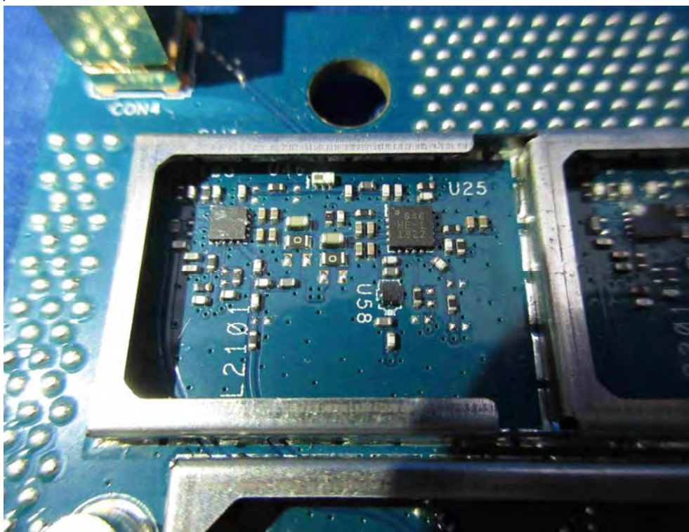
(34) EUT Photo
