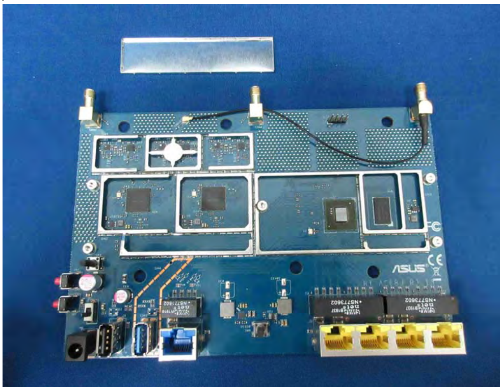
(32) EUT Photo
