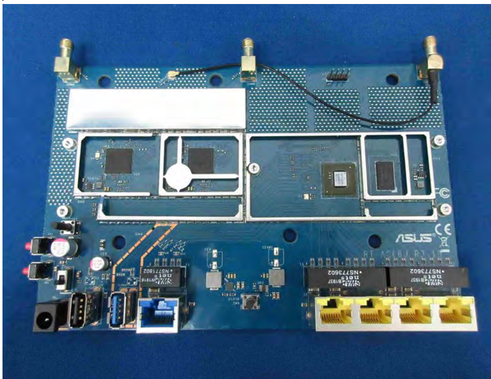
(22) EUT Photo
