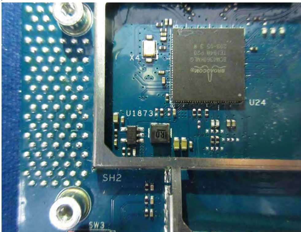
(28) EUT Photo
