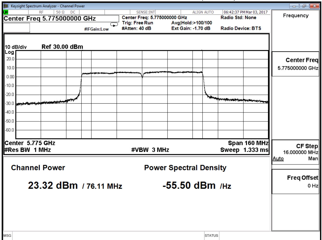
Peak transmit Power - Channel 155 (5775MHz)
