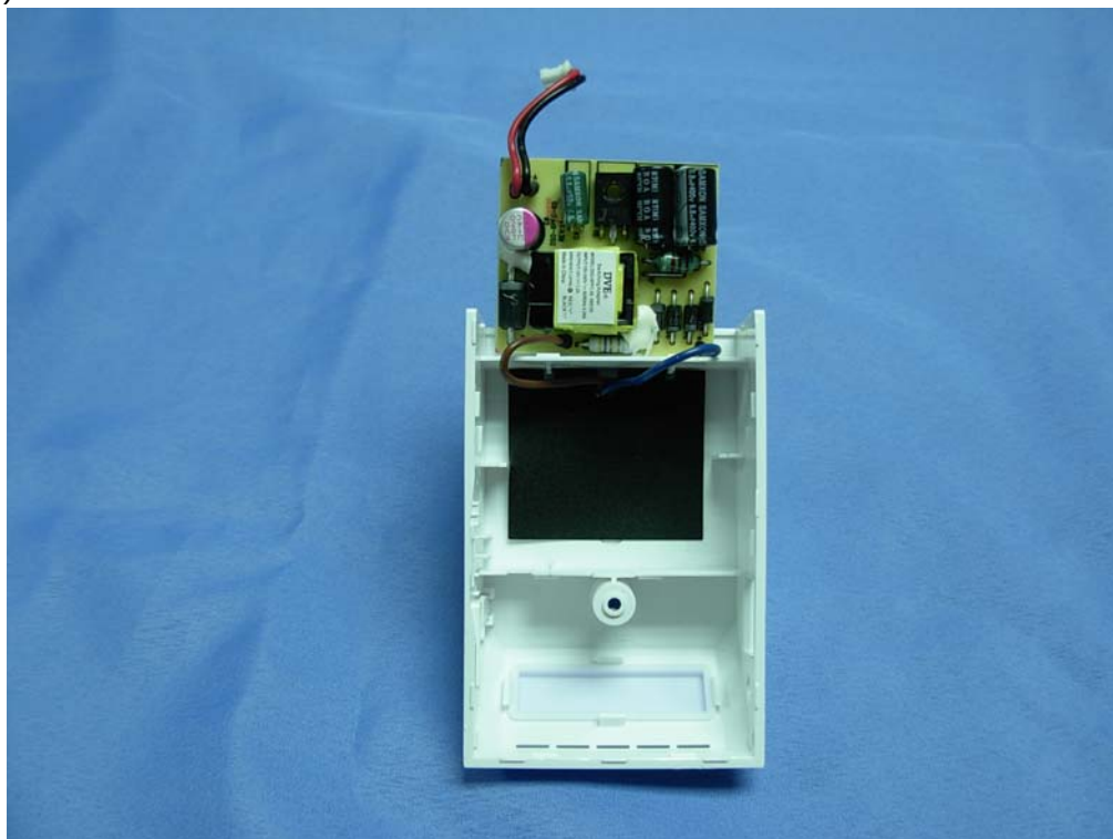
(34) EUT Photo
