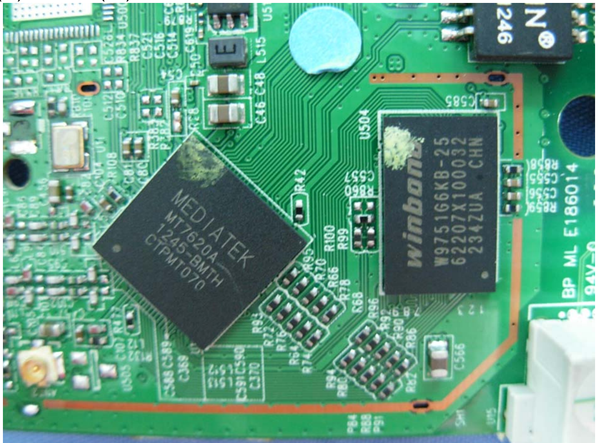
(31) EUT Photo (MB)
