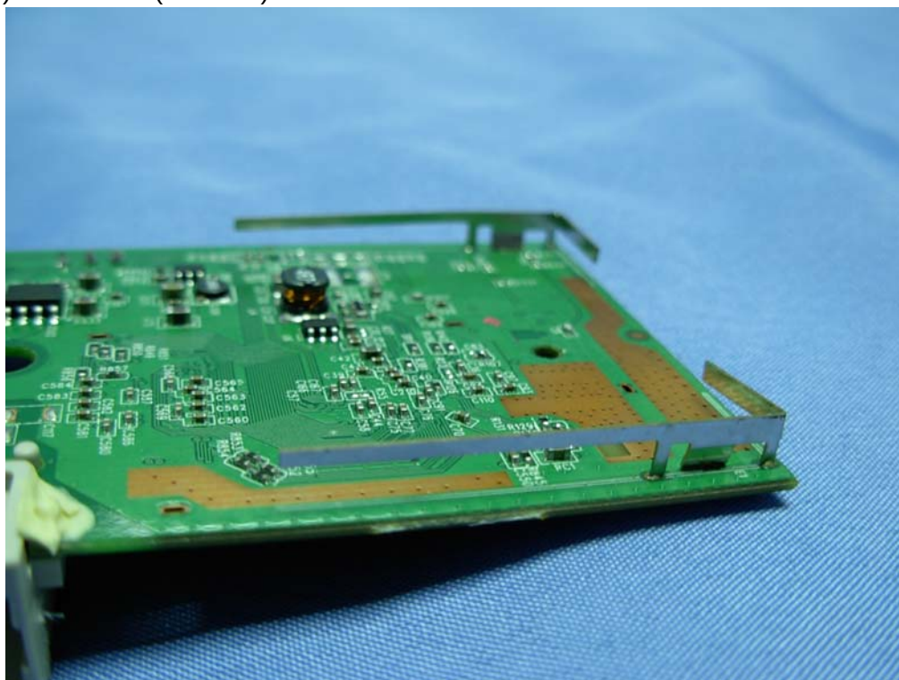
(32) EUT Photo (Antenna)
