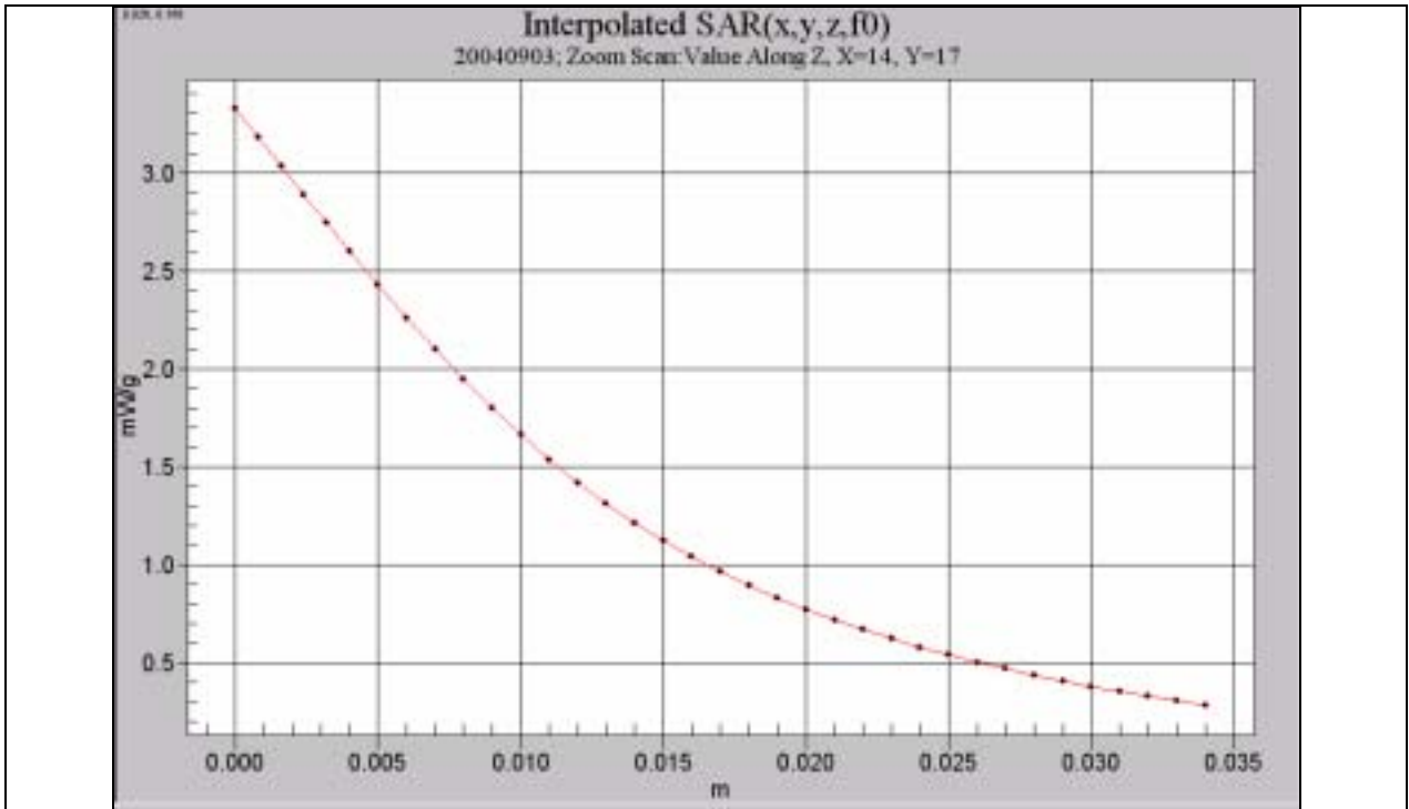
Head-Tissue-Simulating-Liquid 1900MHz
