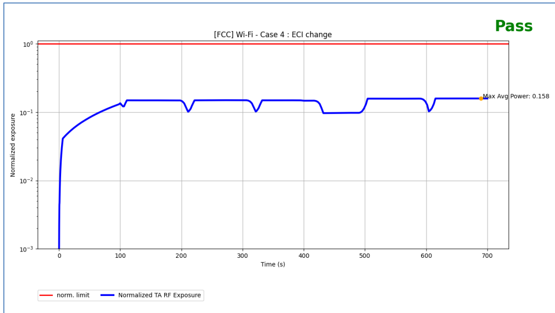
Figure 6-12: Normalized Time-Averaged SAR Over Time for Wi-Fi Test Scenario 4
