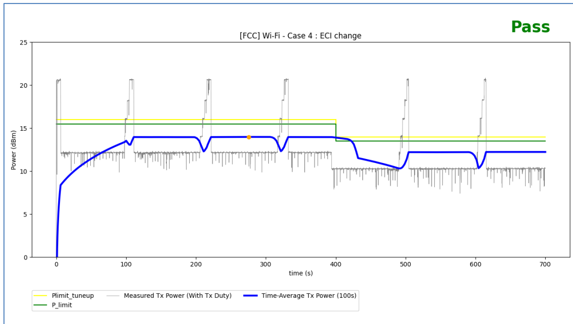
Figure 6-11: Time-Averaged Conducted TX Power Over Time for Wi-Fi Test Scenario 4
