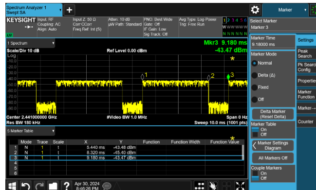
Time-domain Plot for Bluetooth Antenna-1 Transmission
