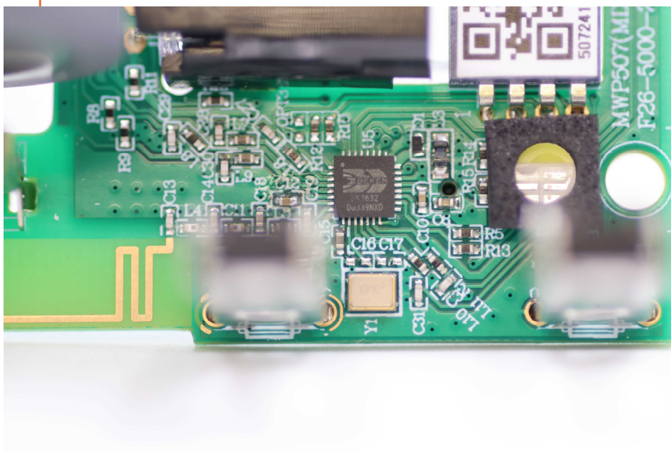
SRD&amp;BLE Antenna
