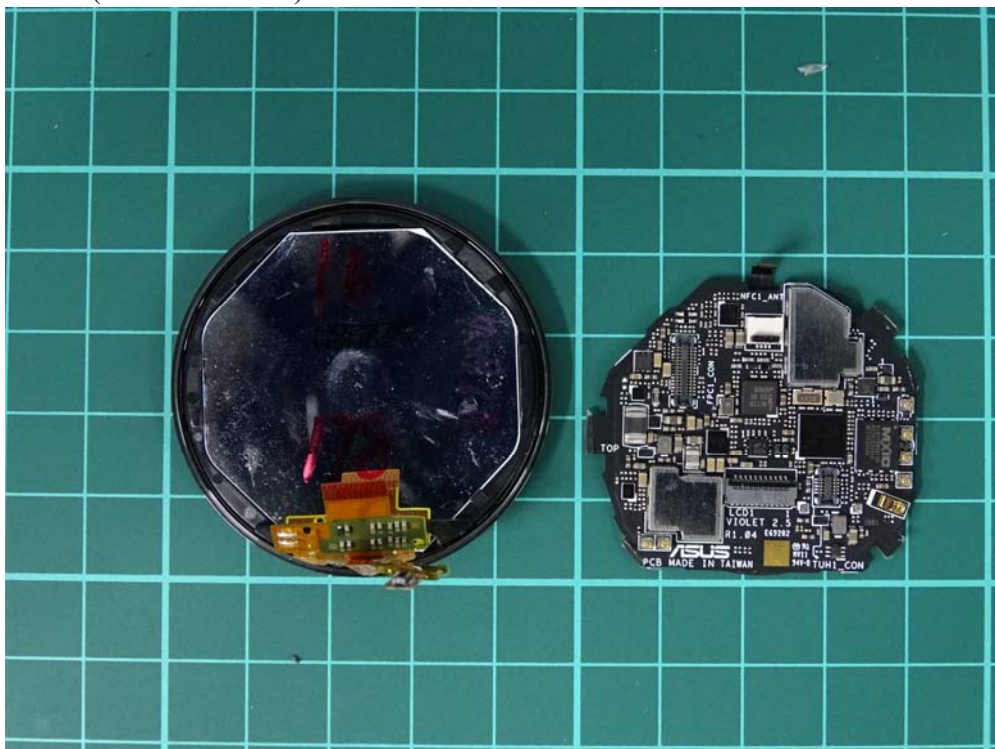
(54) EUT Photo (M/N: HC-A05K)
