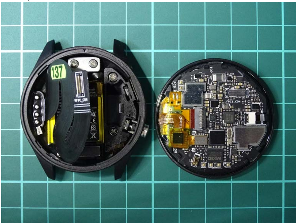
(76) EUT Photo (M/N: MD-A01)
