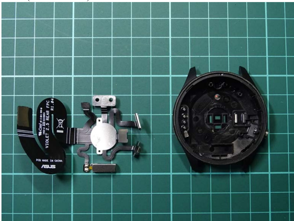
(46) EUT Photo (M/N: HC-A05K)
