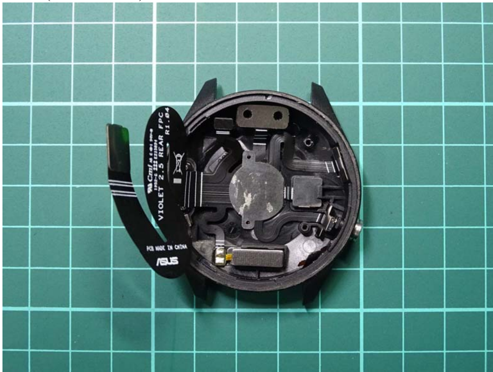
(83) EUT Photo (M/N: MD-A01)
