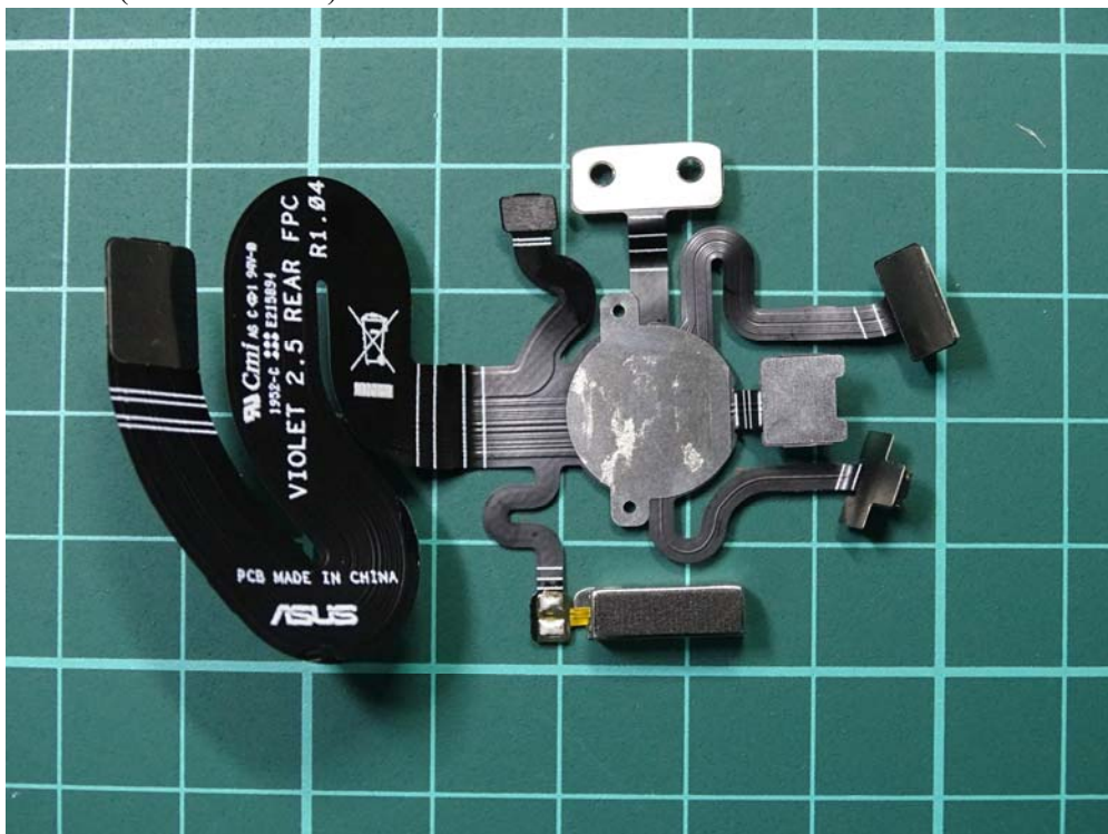
(86) EUT Photo (M/N: MD-A01)
