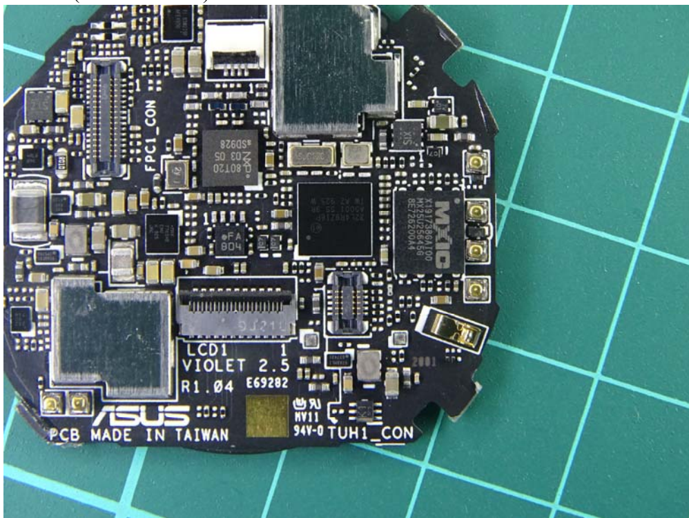
(100) EUT Photo (M/N: MD-A01)
