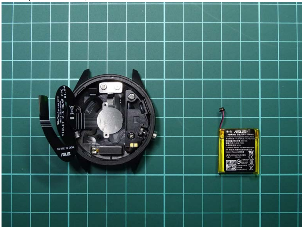
(78) EUT Photo (M/N: MD-A01)
