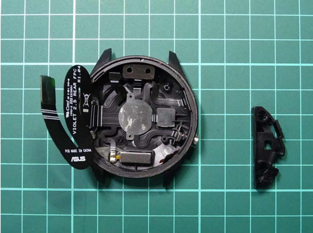
(44) EUT Photo (M/N: HC-A05K)
