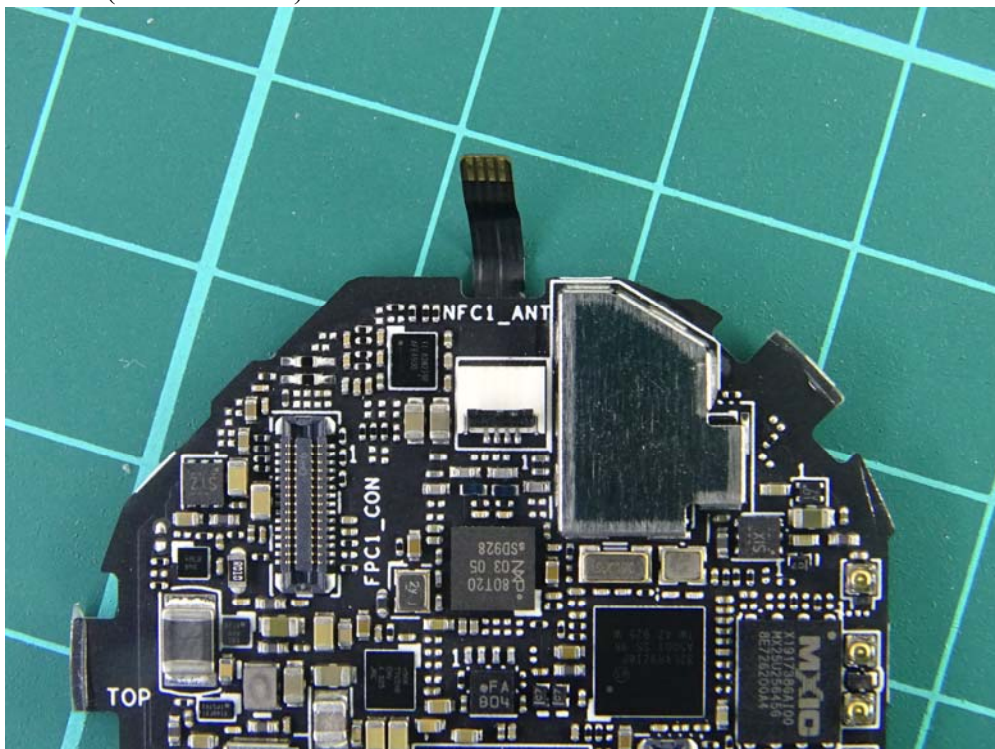
(98) EUT Photo (M/N: MD-A01)
