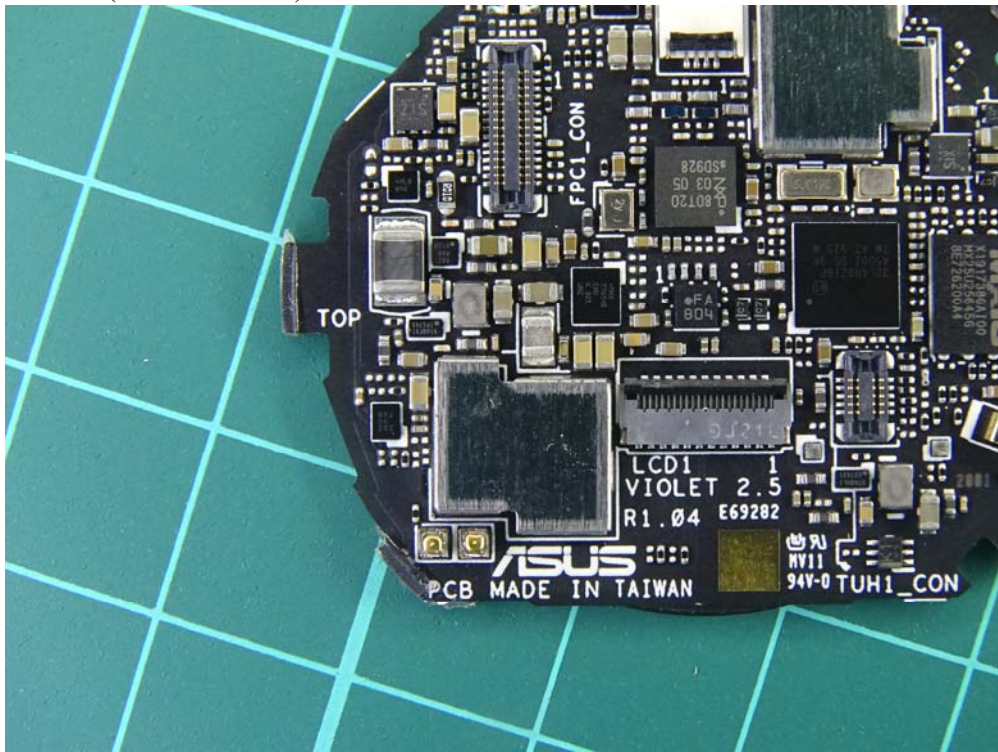
(99) EUT Photo (M/N: MD-A01)
