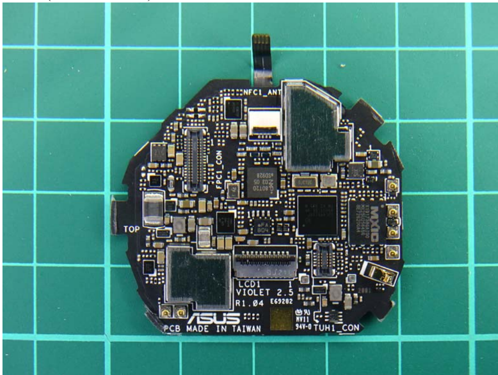
(59) EUT Photo (M/N: HC-A05K)
