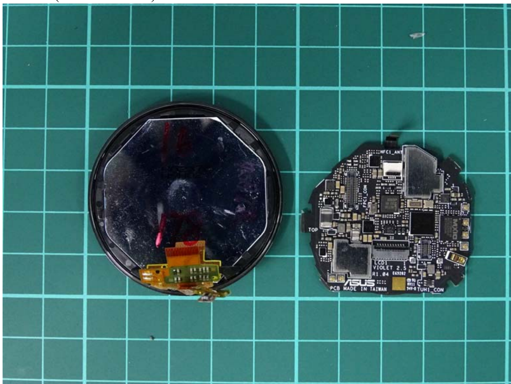
(92) EUT Photo (M/N: MD-A01)
