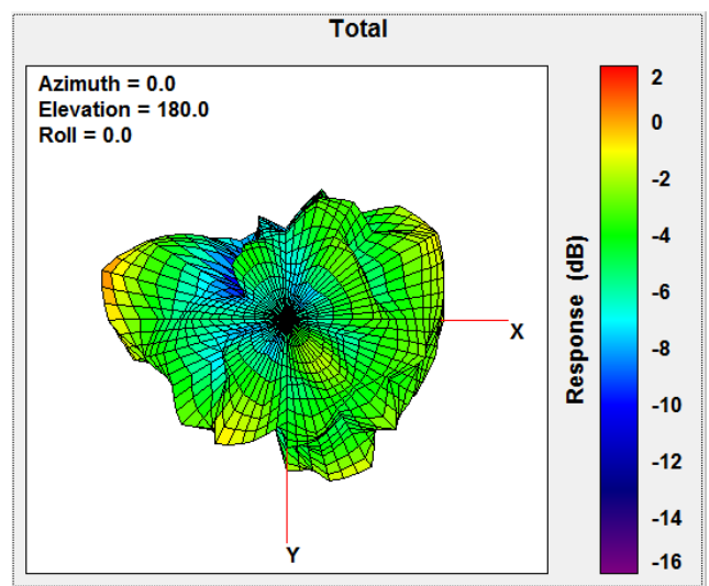
Total Gain Bottom view 2480MHz
