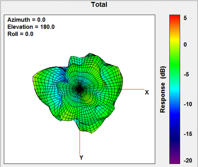
Total Gain Bottom view 2403MHz
