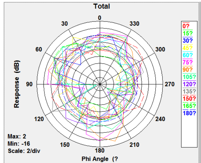
Total Gain Right Side view 2440MHz
