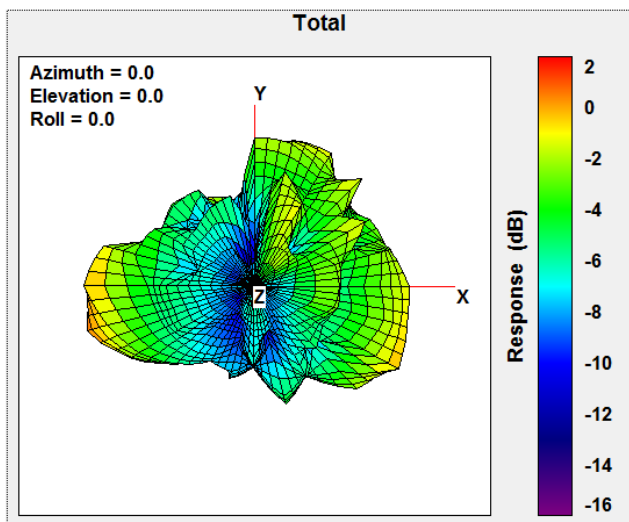
Total Gain Front Face view 2480MHz
