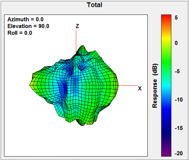
Total Gain Back Face view 2403MHz
