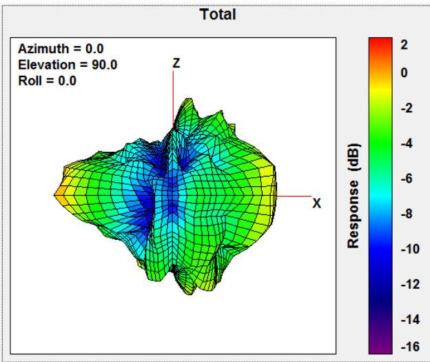
Total Gain Back Face view 2440MHz
