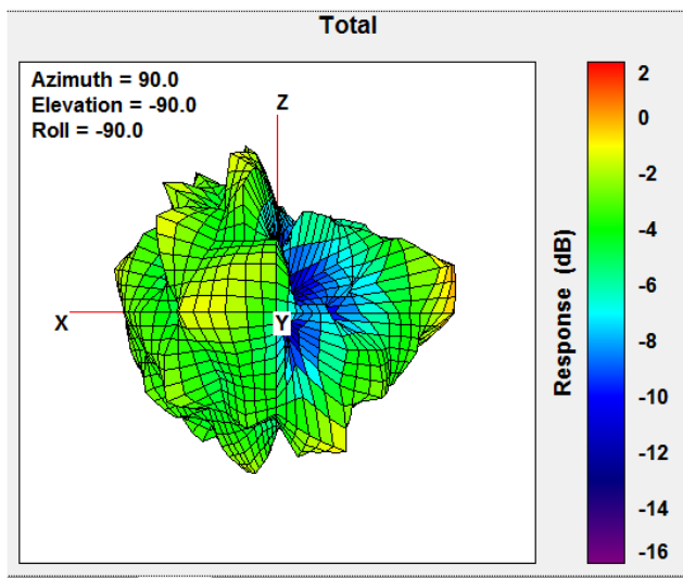
Total Gain Top view 2480MHz
