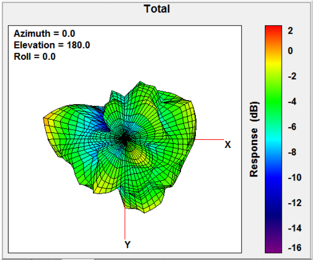
Total Gain Bottom view 2440MHz
