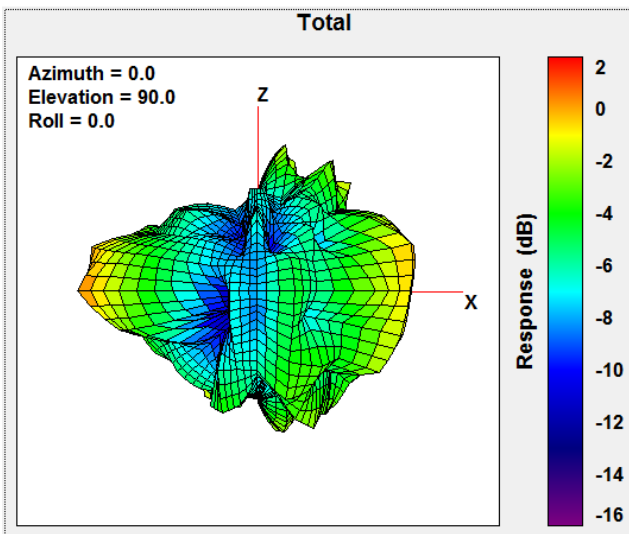
Total Gain Back Face view 2480MHz
