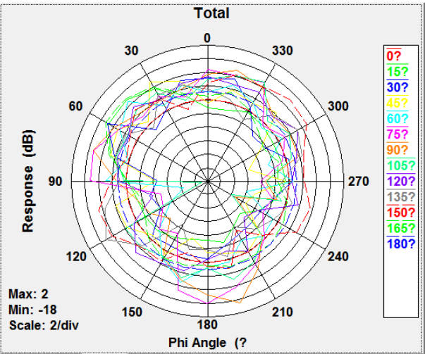
Total Gain Right Side view 2403MHz
