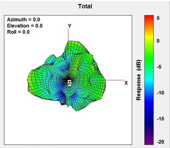
Total Gain Front Face view 2403MHz
