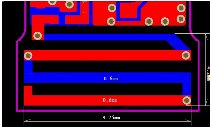
MD102 DG Copper trace antenna dimension 9.75mm(L)*4.2mm(W) Copper 0.5 OZ
