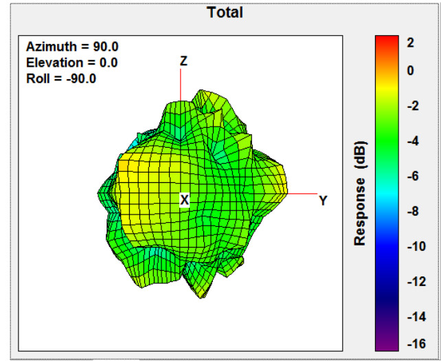
Total Gain Left Side view 2440MHz
