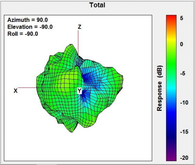
Total Gain Top view 2403MHz
