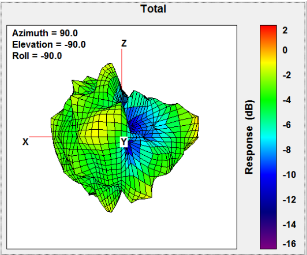
Total Gain Top view 2440MHz
