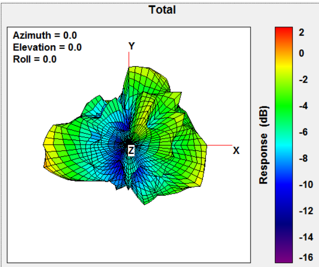
Total Gain Front Face view 2440MHz
