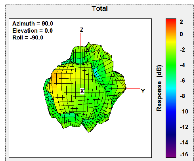
Total Gain Left Side view 2480MHz
