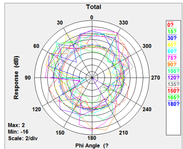
Total Gain Right Side view 2480MHz
