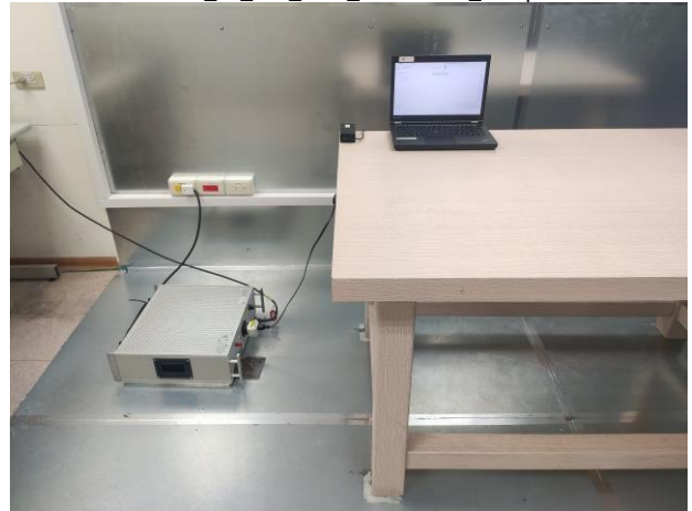
FCC 15_249_SRD_Conduction_Setup
