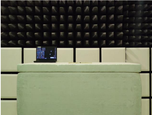
FCC 15_249_SRD_Radiated_Setup
