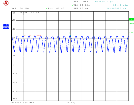
835MHz - 80% AM
