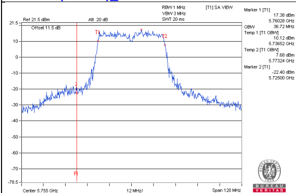
802.11ac(VHT40)_Chain2 / CH151
