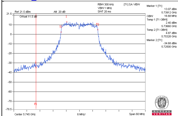
802.11ac(VHT20)_Chain0 / CH149
