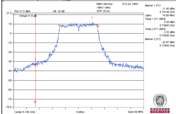
802.11ac(VHT20)_Chain2 / CH149
