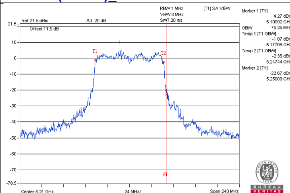
802.11ac(VHT80)_Chain0 / CH42
