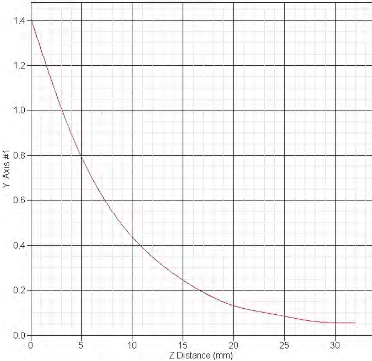
SAR-Z Axis at Hotspot x:28.20 y:-5.80
