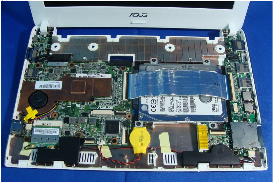
(7) EUT Photo
