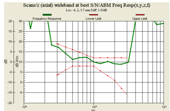
Fig. 9.4 GSM1900 Ch512
