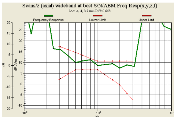
Fig. 9.5 GSM1900 Ch661
