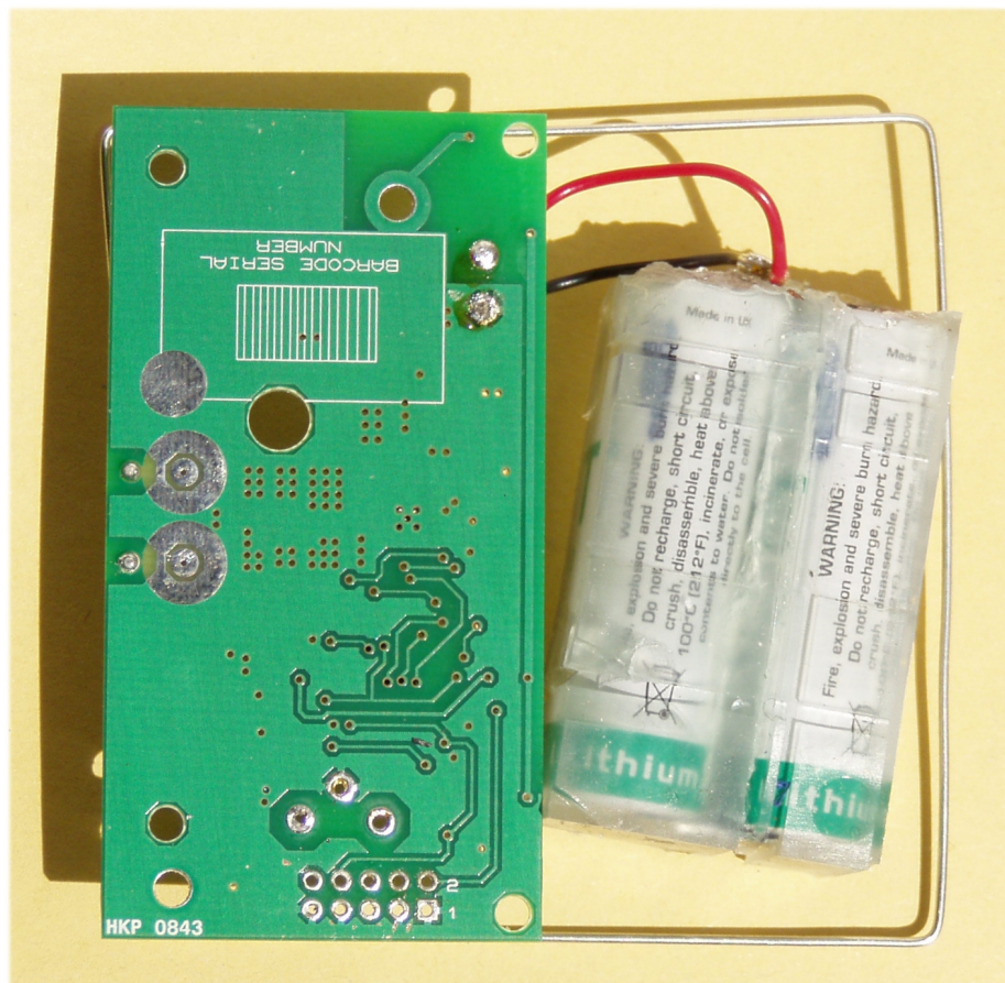
BOTTOM VIEW
