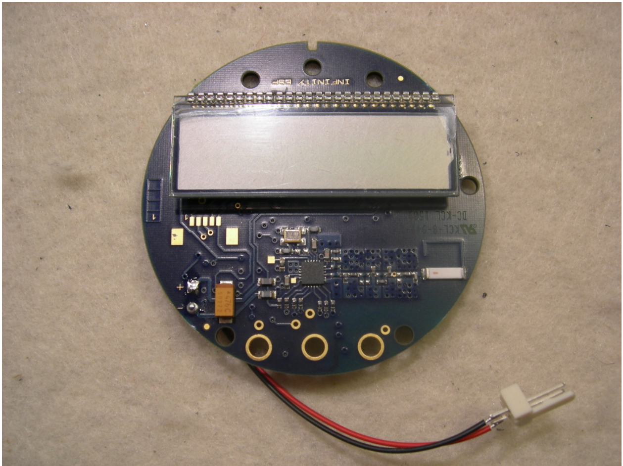
Figure 1: PCB - Front
