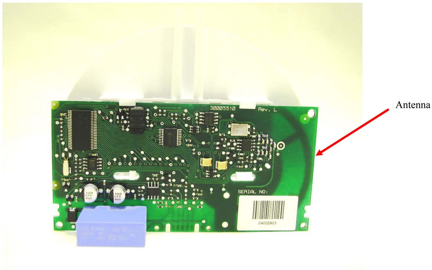
Figure 2: Rear view of TransPondIT Centron 120V module - showing PCB antenna position
