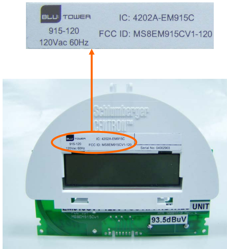
Figure 1: TransPondIT Centron 120V module (removed from meter): LCD front view
