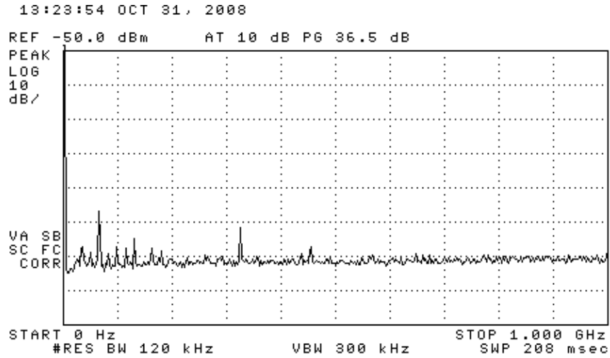
Figure 6.1. Emissions measured at 3 meters in chamber, 0-1000 MHz.
