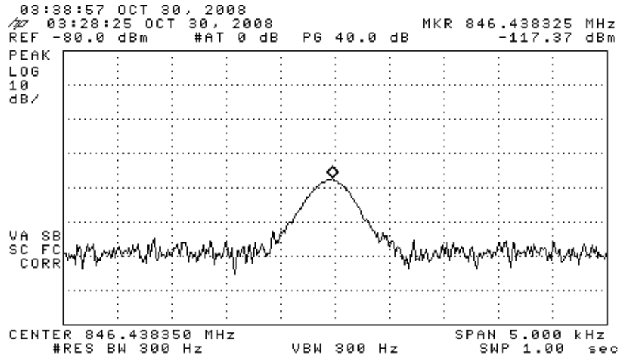
Figure 6.3. Relative receiver emission(s).
