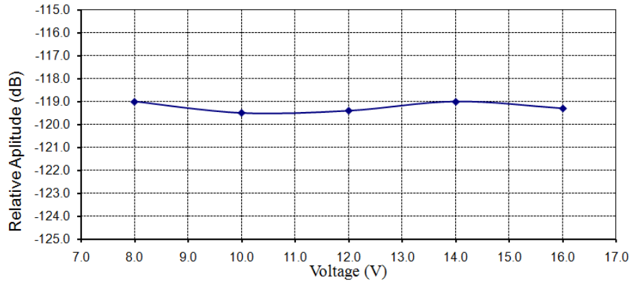
Figure 6.4. Relative emission vs. supply voltage.
