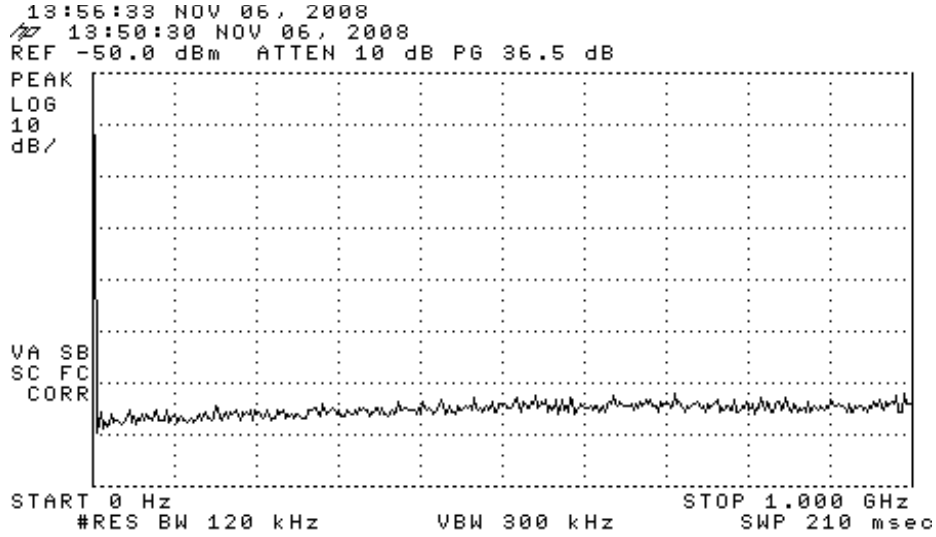
Figure 6.1. Emissions measured at 3 meters in chamber, 0-1000 MHz.
