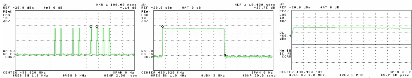
Figure 5(c): Pulsed Emission Characteristics (Duty Cycle).
