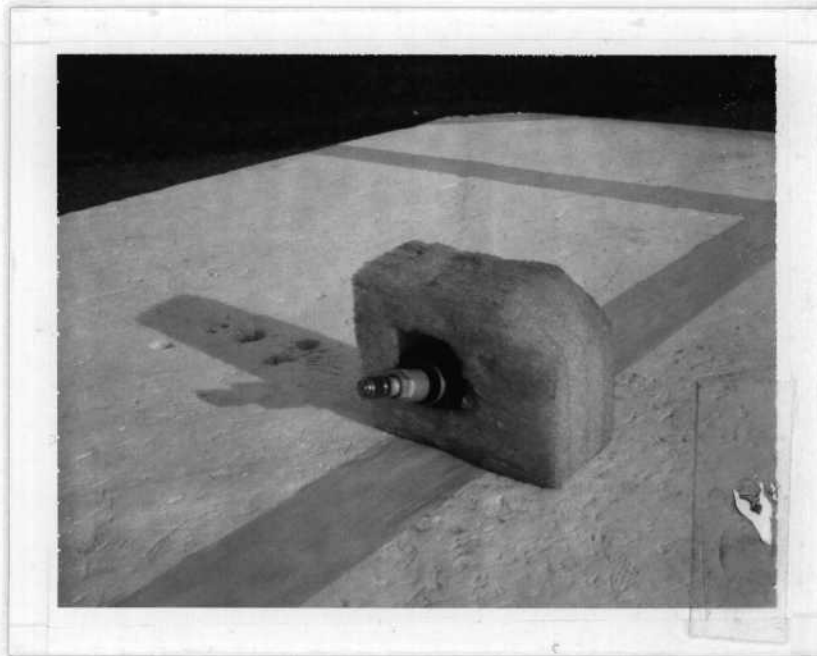
Appendix: DUT on the test table (Open-Site). (top) Overall view (bottom) Close-up
