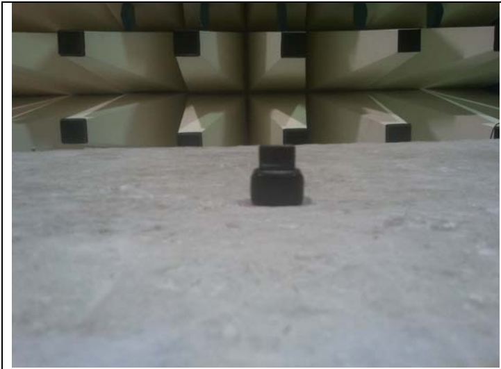
Fig 3 Test setup
