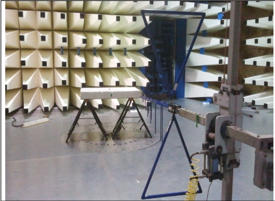
Fig 1 Test setup
