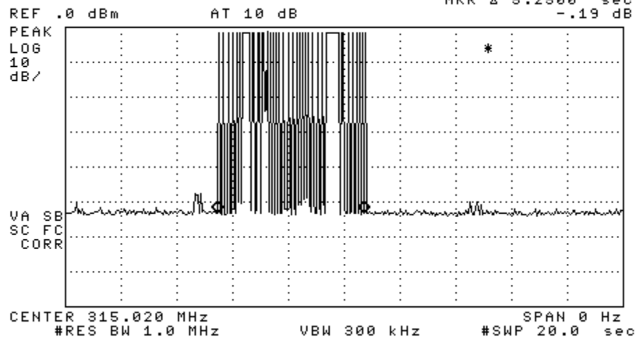
Figure 6.1(a). Transmissions modulation characteristics: (top) Drive Mode, (center) Factory Mode, (bottom) LF interrogation response.
