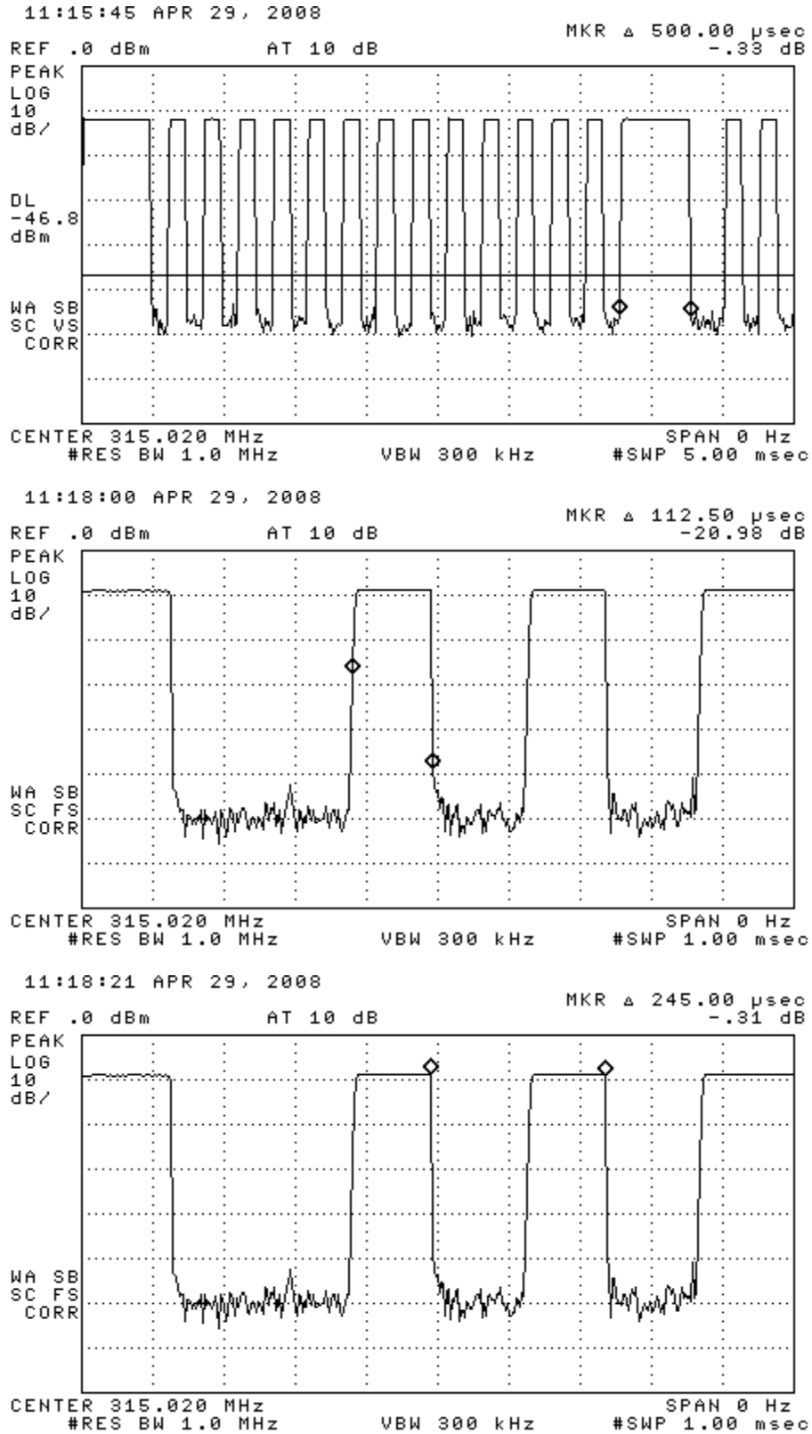
Figure 6.1(c). Transmissions modulation characteristics: (top) expanded word, (center) Manchester bit, (bottom) Manchester period.
