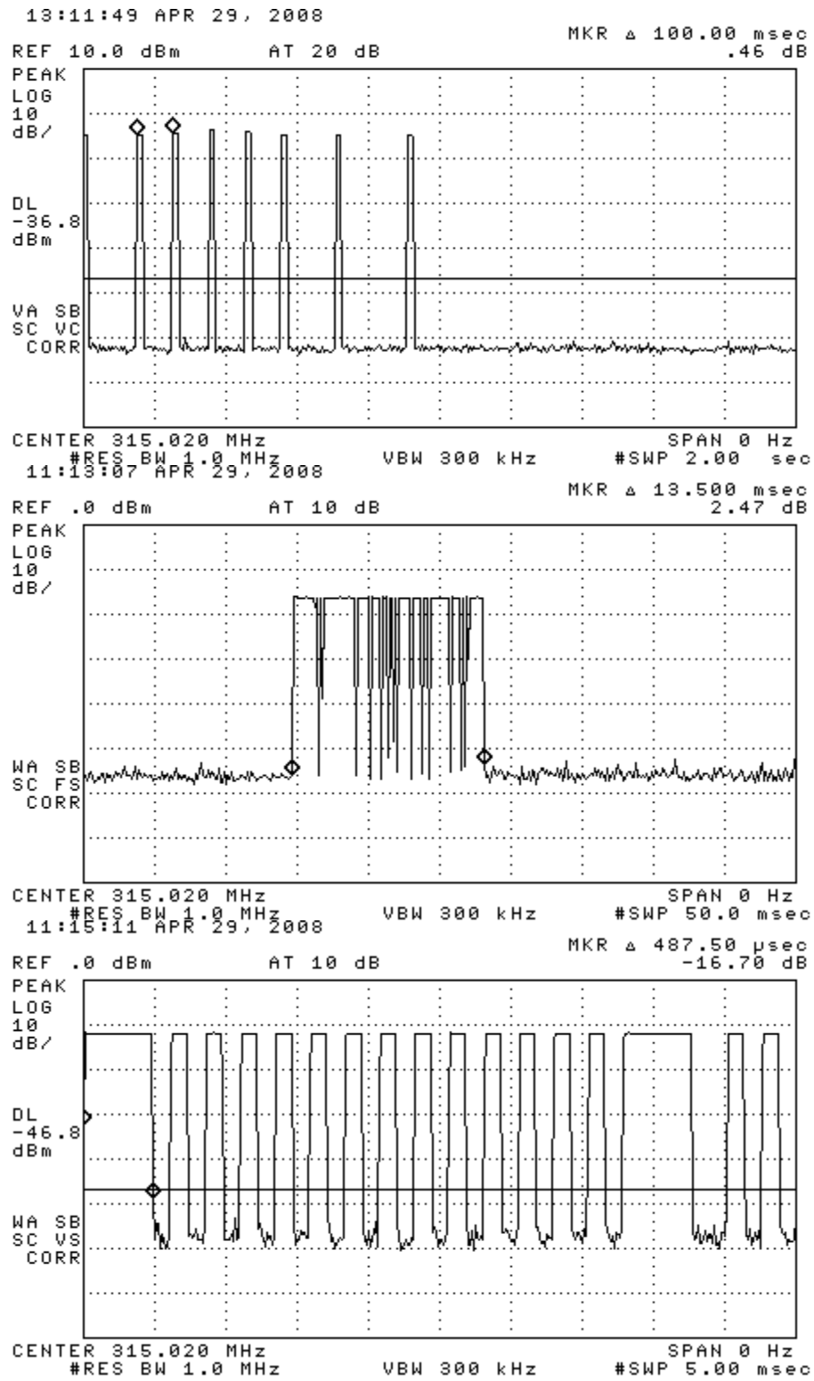
Figure 6.1(b). Transmissions modulation characteristics: (top) minimum word separation, (center) single word, (bottom) expanded word.
