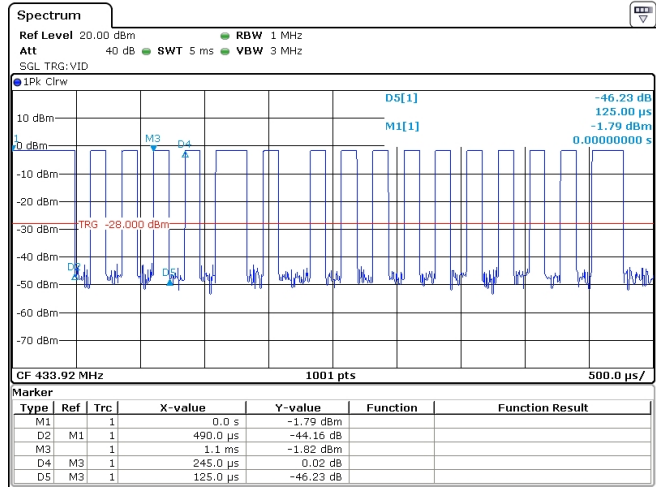
Figure 5(a): Pulsed Emission Characteristics (Duty Cycle).
