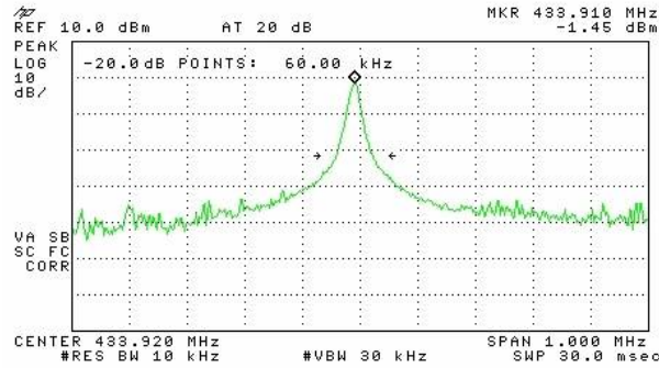
Figure 6: Intentional Emission Bandwidth.
