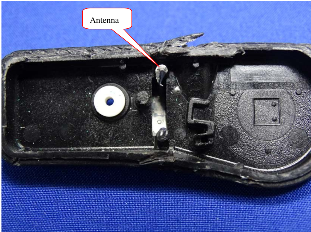
(12) EUT Photo-Antenna
