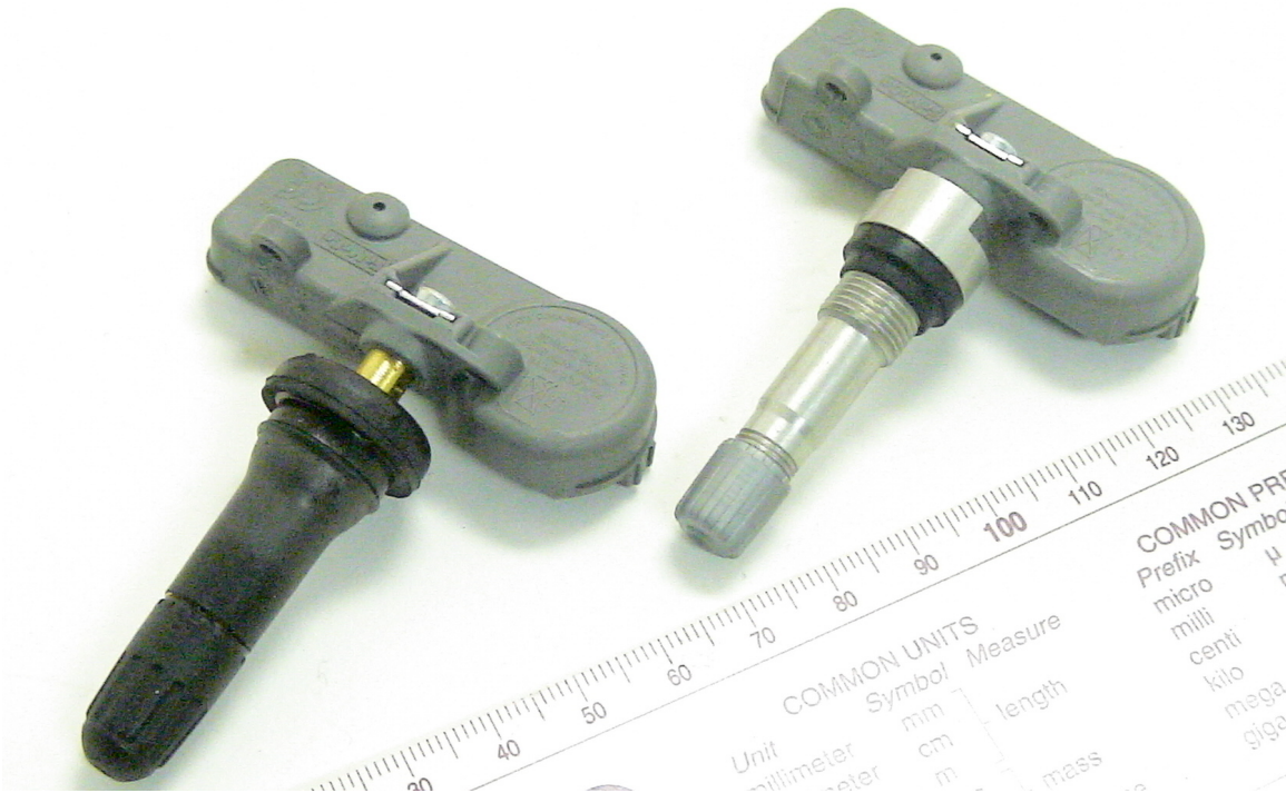
Figure 1: Photographs of the EUT.
