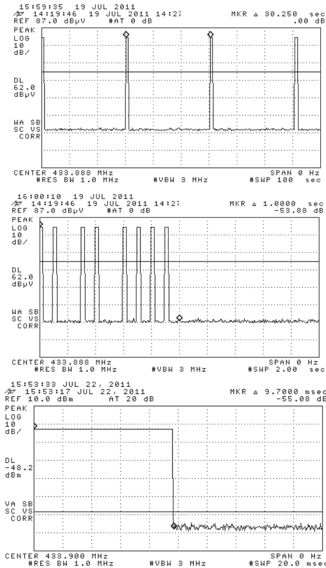
Figure 5(b): Pulsed Emission Characteristics (Duty Cycle).
