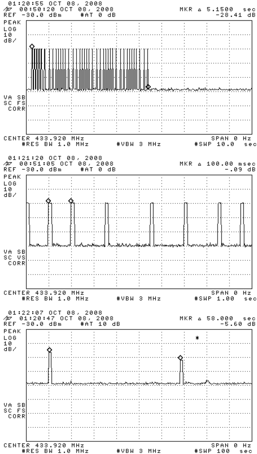
Figure 6.1(a). Transmission modulation characteristics. (top) response to manual LF interrogation, (center) minimum word period (true for all modes), (bottom) roll-mode transmission.
