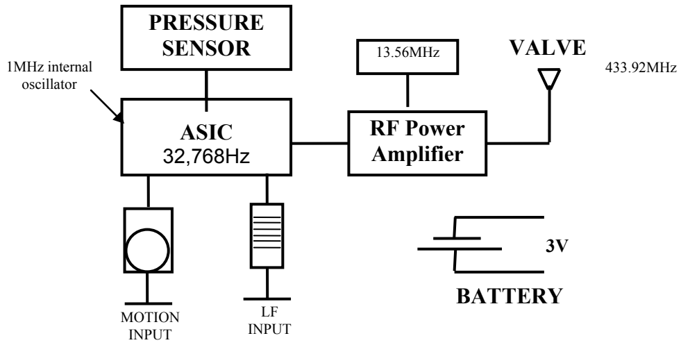
Nissan JY00B Block Diagram
