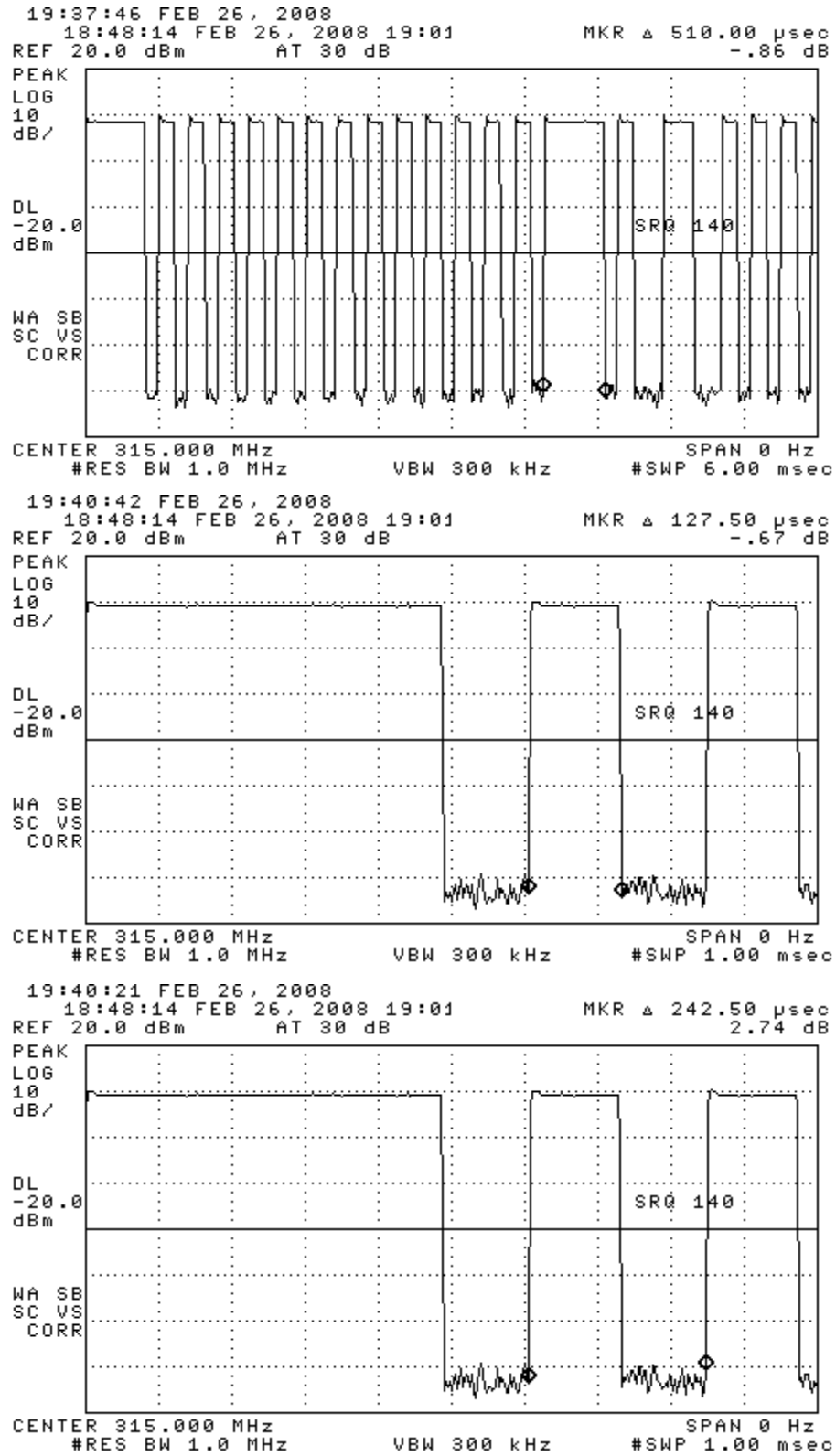
Figure 6.1(b). Transmissions modulation characteristics: (top) data lead pulse, (center) Manchester pulse width, (bottom) pulse period.
