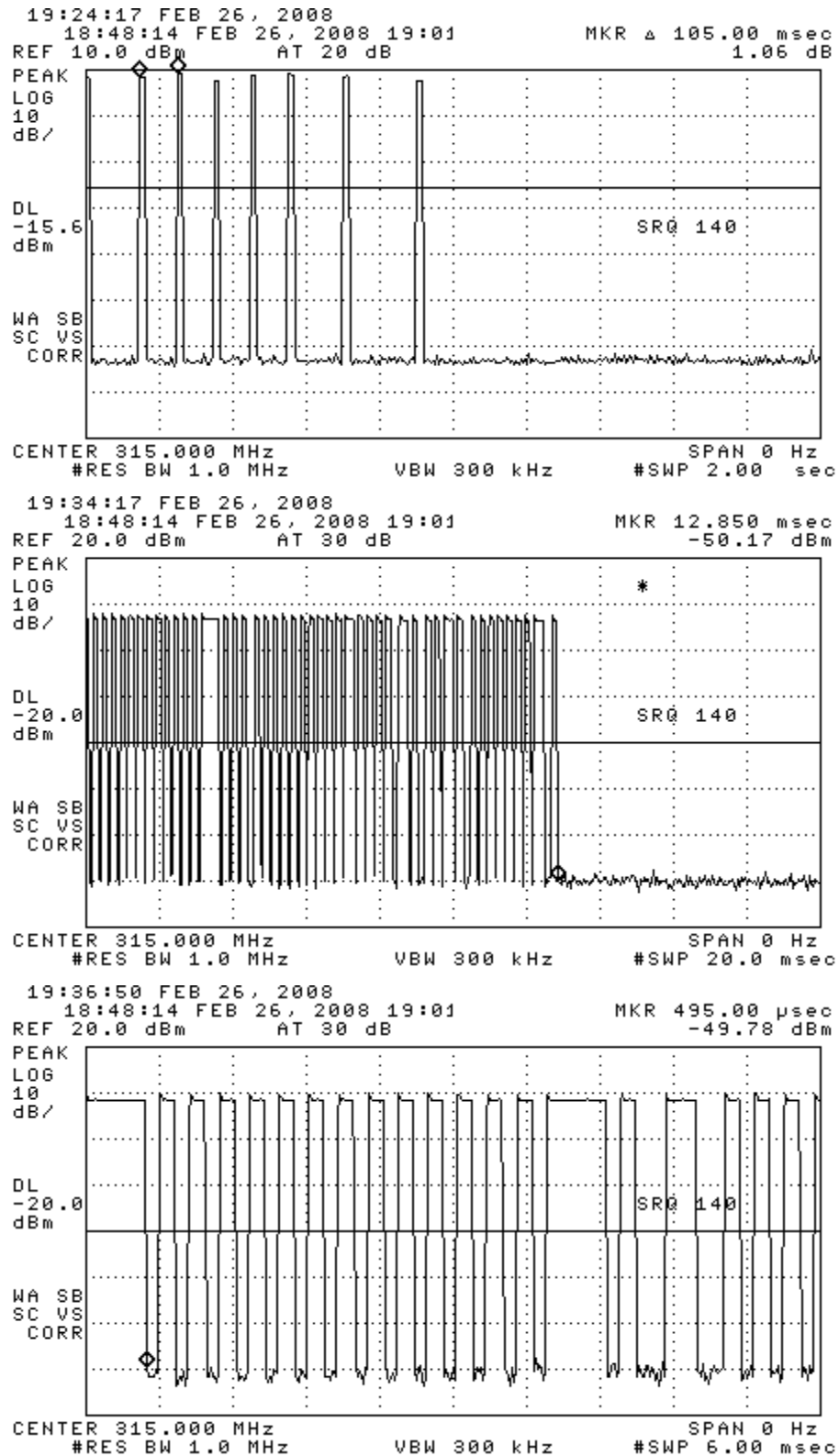
Figure 6.1(a). Transmissions modulation characteristics: (top) complete ID Response transmission, (center) transmitted word, (bottom) wake pulse width.
