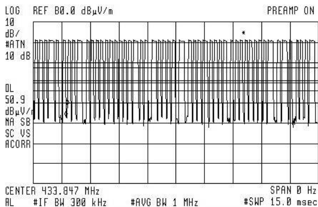
Figure 5(a): Fundamental Emission Pulsed Operation.
