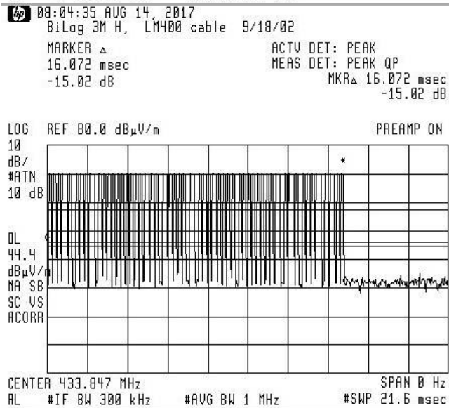
Figure 5(b): Fundamental Emission Pulsed Operation.
