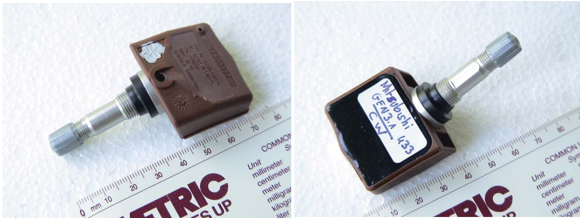
Figure 1: Photographs of the EUT.
