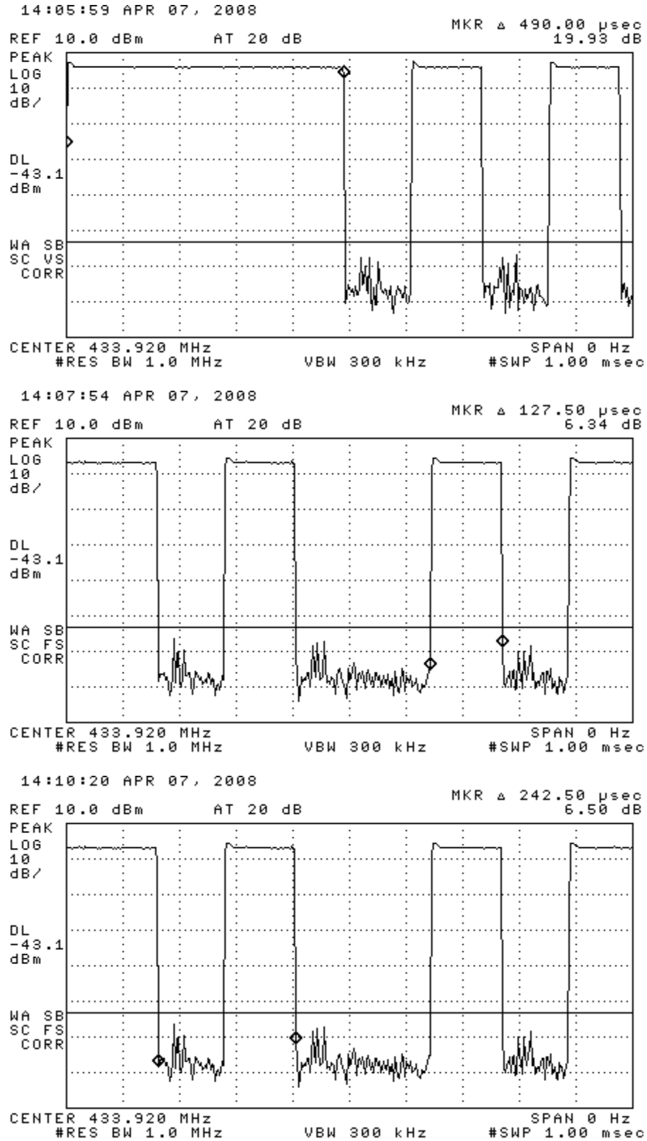
Figure 6.1(c). Transmissions modulation characteristics: (top) Wake pulse, (center) Manchester pulse width, (bottom) Manchester period.
