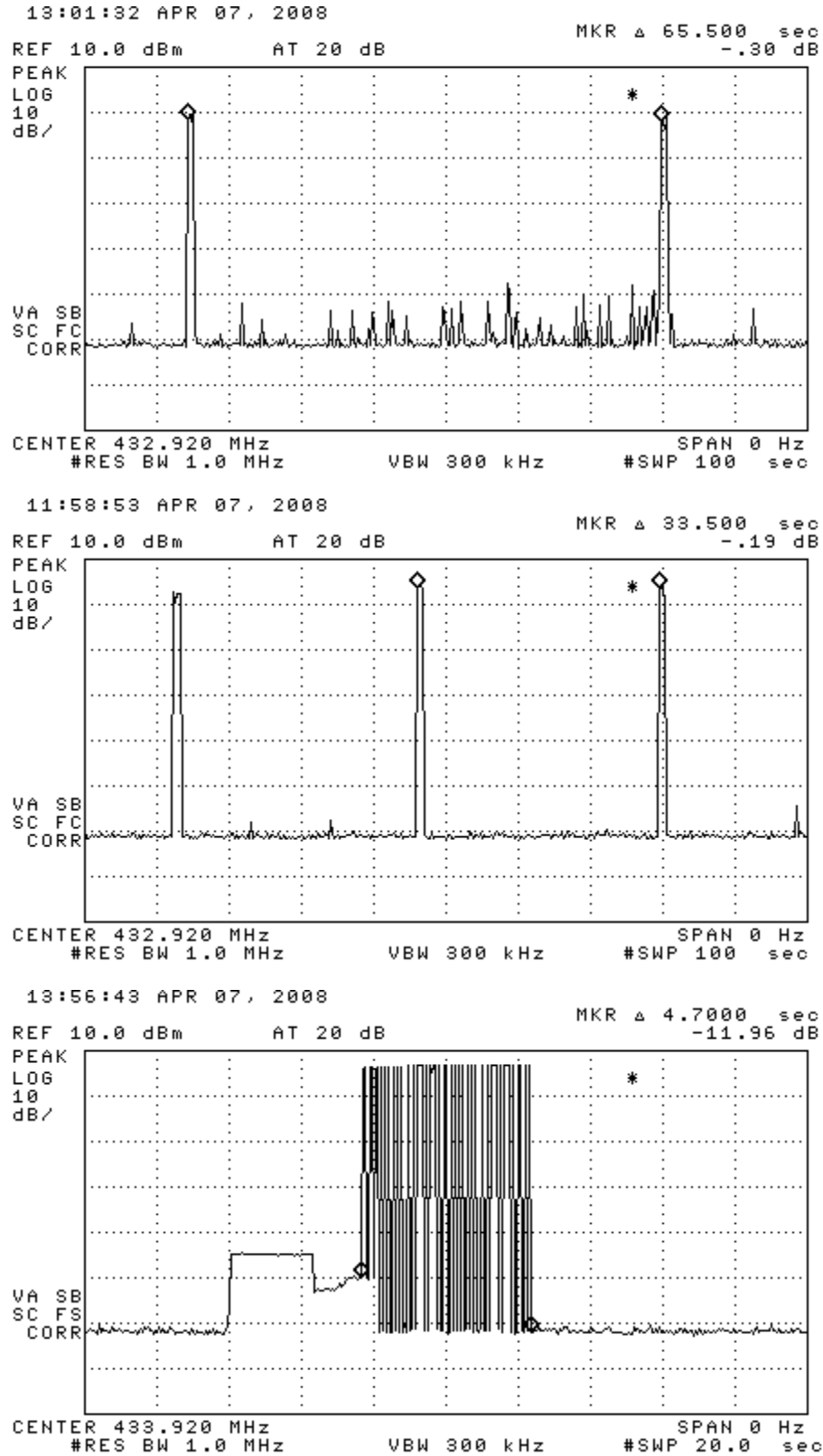
Figure 6.1(a). Transmissions modulation characteristics: (top) Normal Drive Mode complete transmission, (middle) WAL Drive Mode complete transmission, (bottom) LF Interrogation complete transmission
