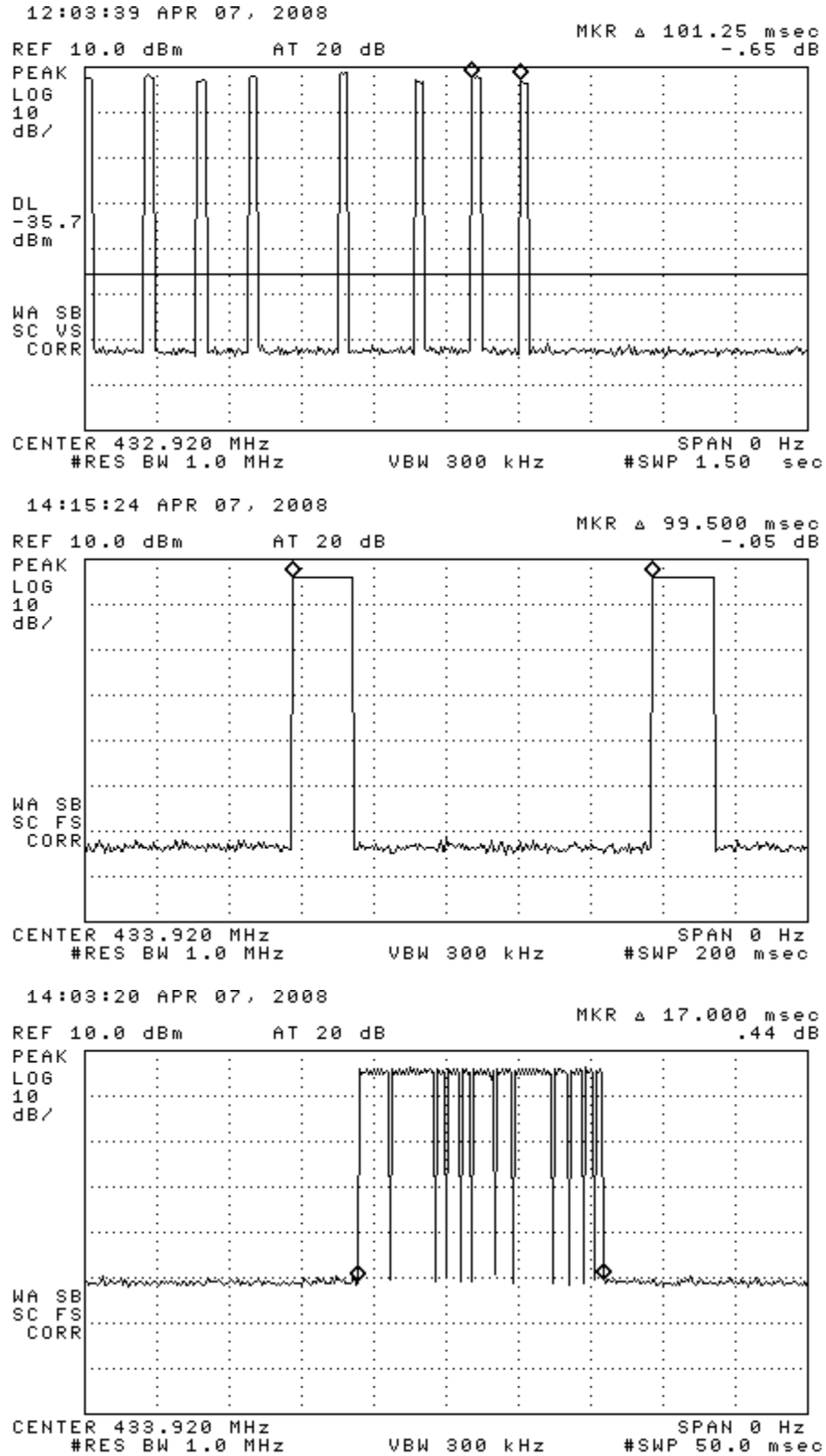
Figure 6.1(b). Transmissions modulation characteristics: (top) worst case complete transmission, (center) worst case word period in transmission, (bottom) single word.
