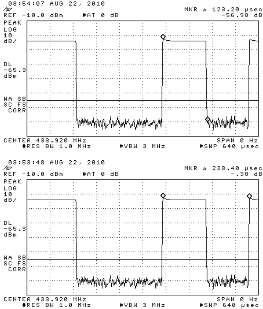
Figure 6.1(c). Transmission characteristics. (top) Manchester pulse width, (bottom) Manchester pulse period.
