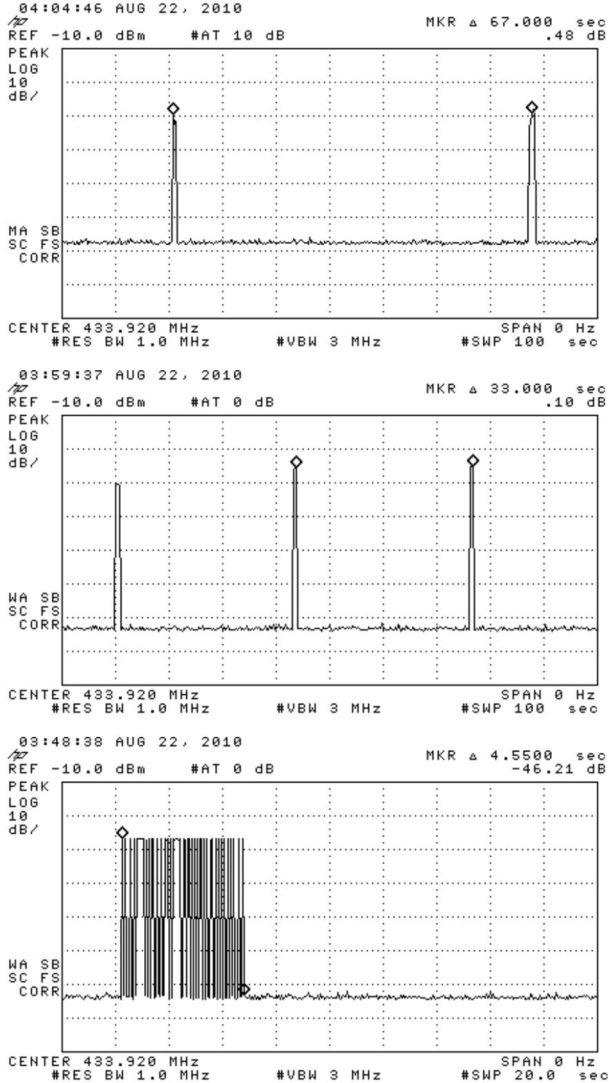
Figure 6.1(a). Transmission modulation characteristics. (top) Normal Drive Mode complete transmission, (middle) WAL Drive Mode complete transmission, (bottom) LF Interrogation complete transmission
