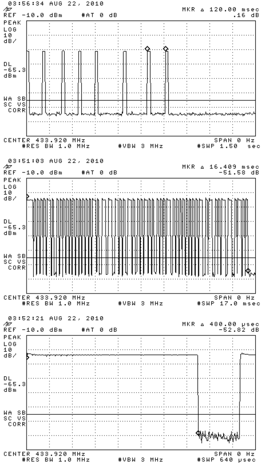
Figure 6.1(b). Transmission modulation characteristics. (top) worst case repeated frames, (middle) frame length, (bottom) leading wake pulse length.
