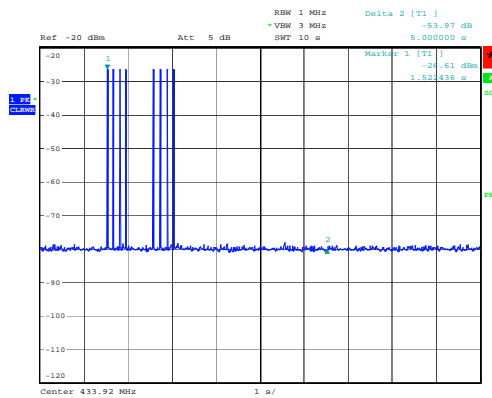
(a) a-LEARN-MODE-LESS-THAN-5-SEC-ON-TIME
