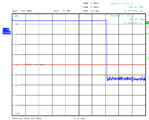
(a) a-LEARN-MODE-LESS-THAN-5-SEC-ON-TIME
