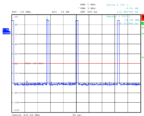
(c) c-LEARN-MODE-SINGLE-FRAME
