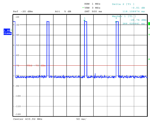
(b) b-LEARN-MODE-FOUR-FRAMES
