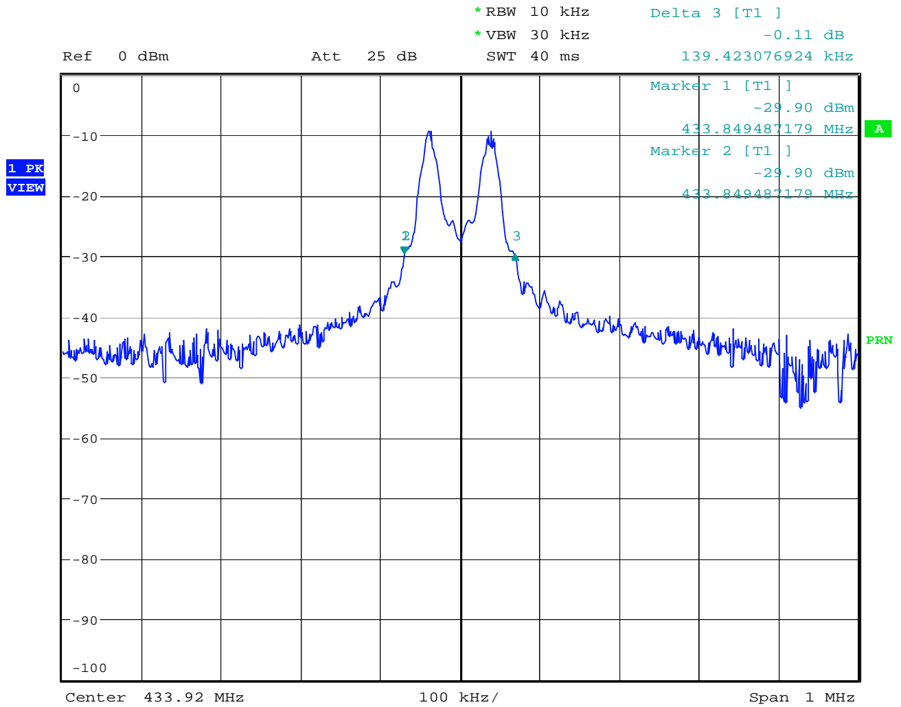
Figure 6: Intentional Emission Bandwidth.
