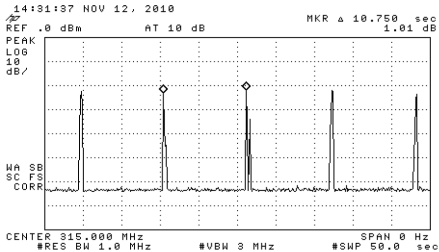
Figure 6.1(b). Drive Mode periodic transmission modulation characteristics. Minimum transmission period.
