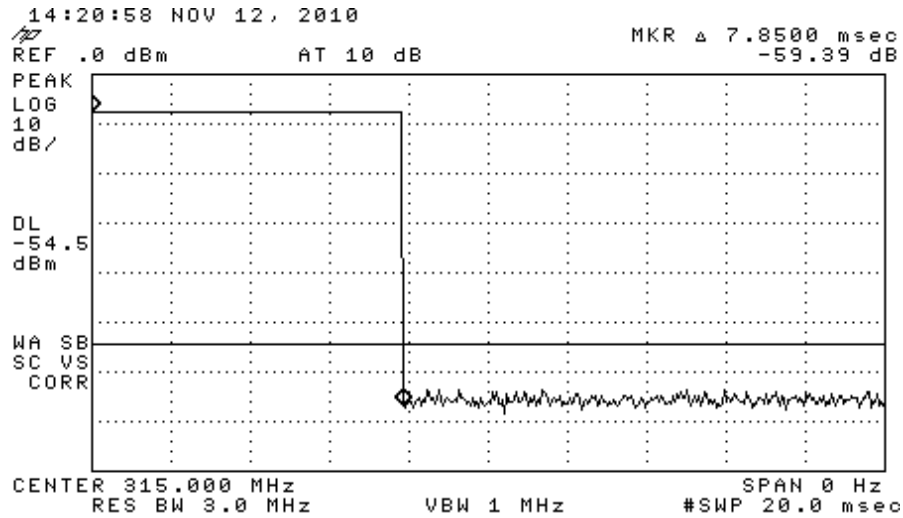
Figure 6.1(a). LF activated manual transmission modulation characteristics. (top) single LF interrogated transmission, (center) minimum frame period, (bottom) FSK frame length.
