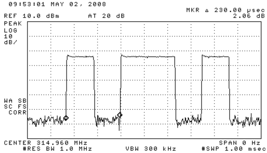
Figure 6.1(c). Transmissions modulation characteristics: Manchester period,
