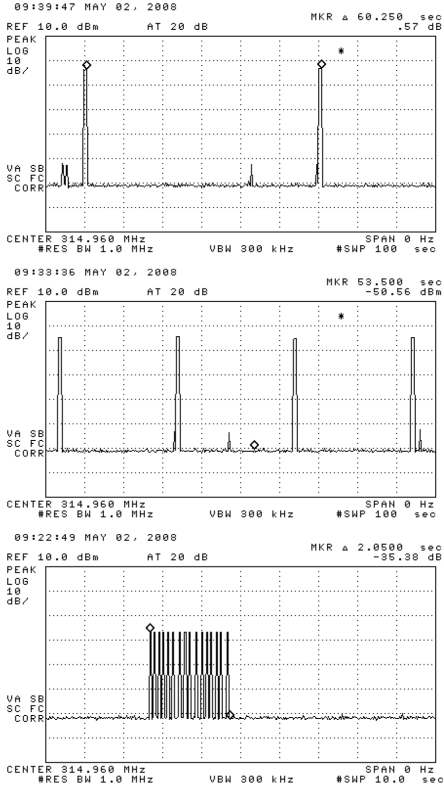
Figure 6.1(a). Transmissions modulation characteristics: (top) Drive Mode, (center) Factory Mode, (bottom) Learn Mode.
