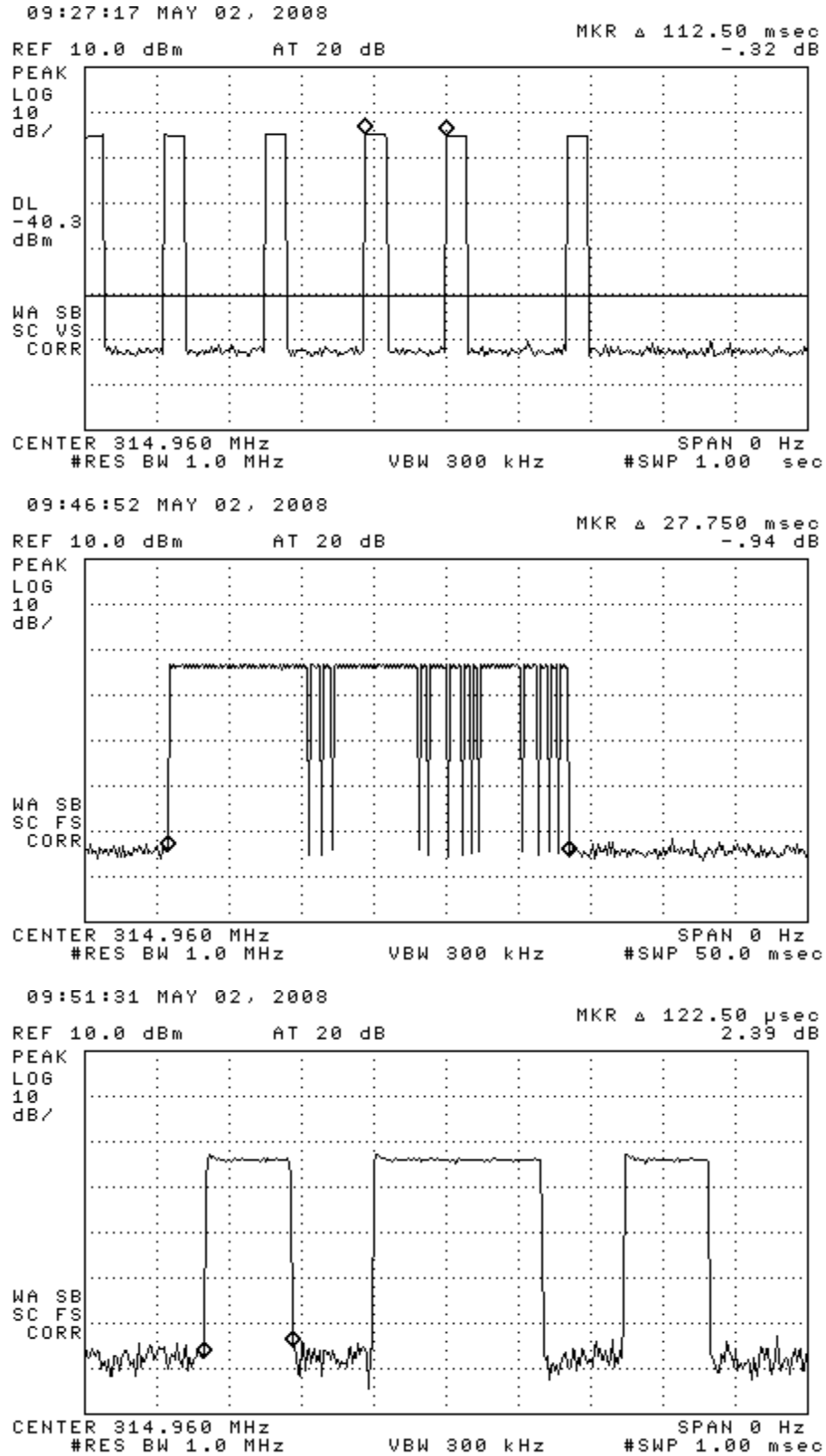
Figure 6.1(b). Transmissions modulation characteristics: (top) one transmission, (center) expanded word, (bottom) Manchester on-time.
