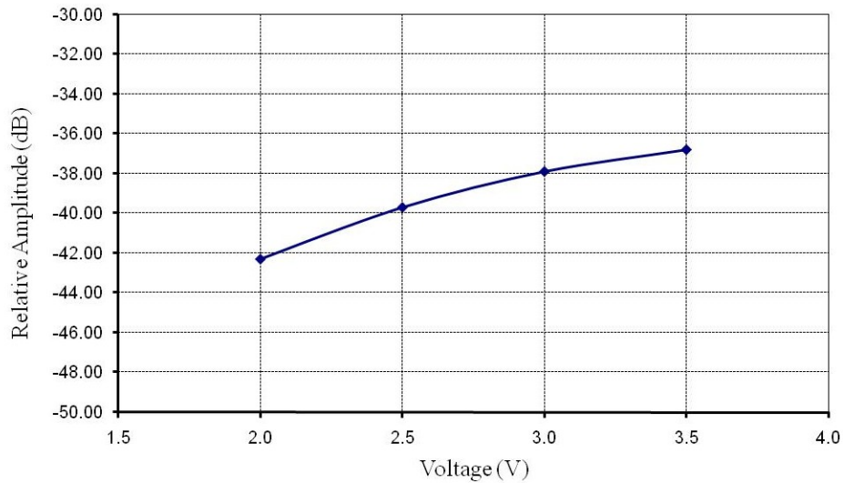
Figure 6.4. Relative emissions at 315 MHz vs. supply voltage. (cw emission)
