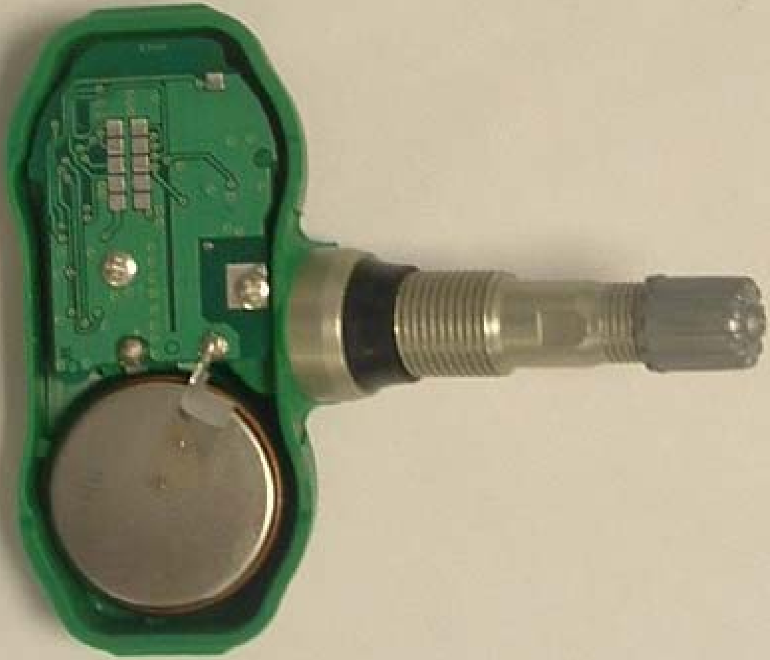
DUT unpotted (bottom)
