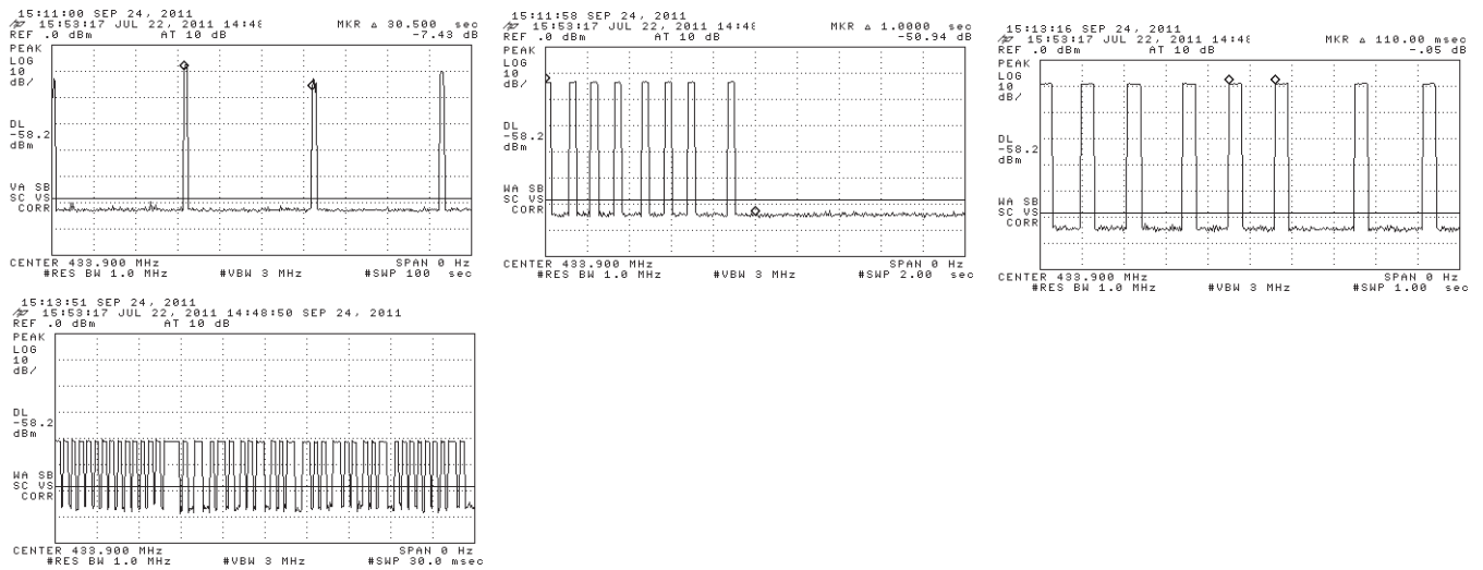
Figure 5(b): Pulsed Emission Characteristics (Duty Cycle).
