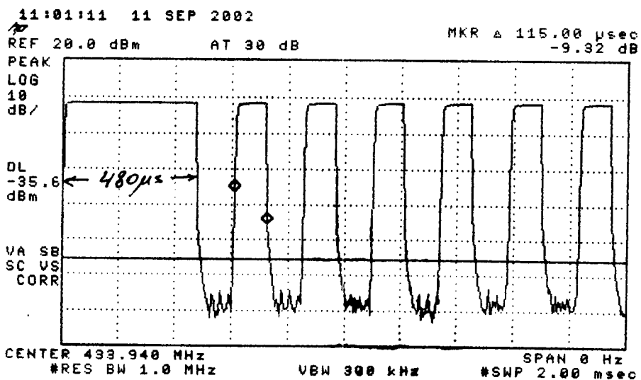
Figure 6.1. Transmissions modulation characteristics: (top) transmission repetition, (center) transmission pulses, (bottom) pulse widths.
