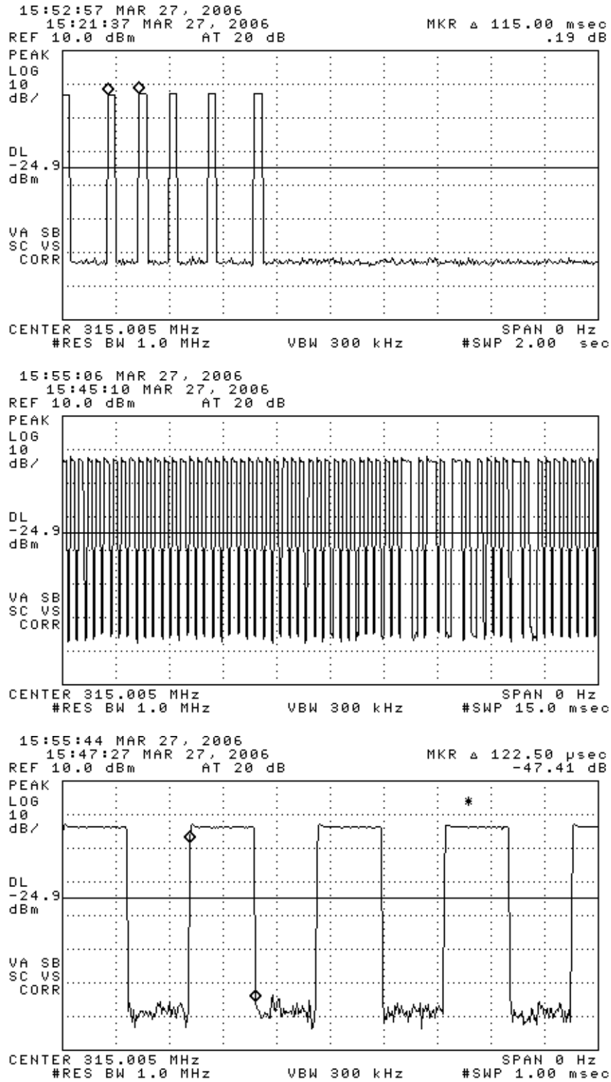
Figure 6.1. Transmissions modulation characteristics: (top) complete transmission, (center) expanded transmission, (bottom) expanded word.
